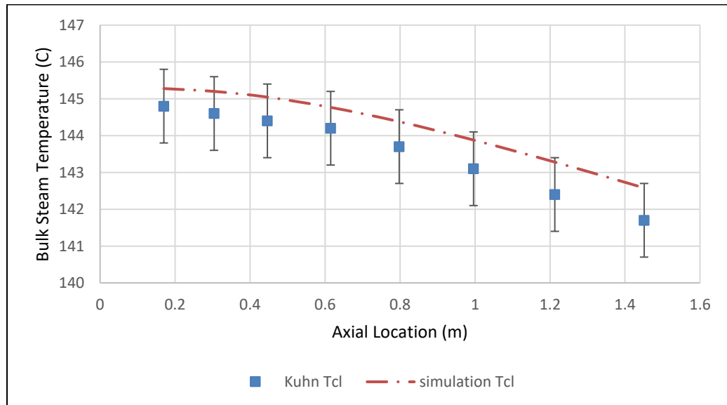
Figure 5.9 Bulk temperatures for Kuhn2.1-8R run on steam region
