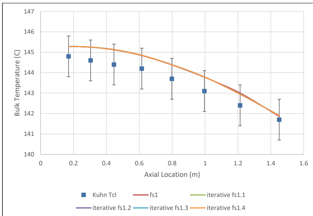
Figure 5.12 Iterative study results for steam
