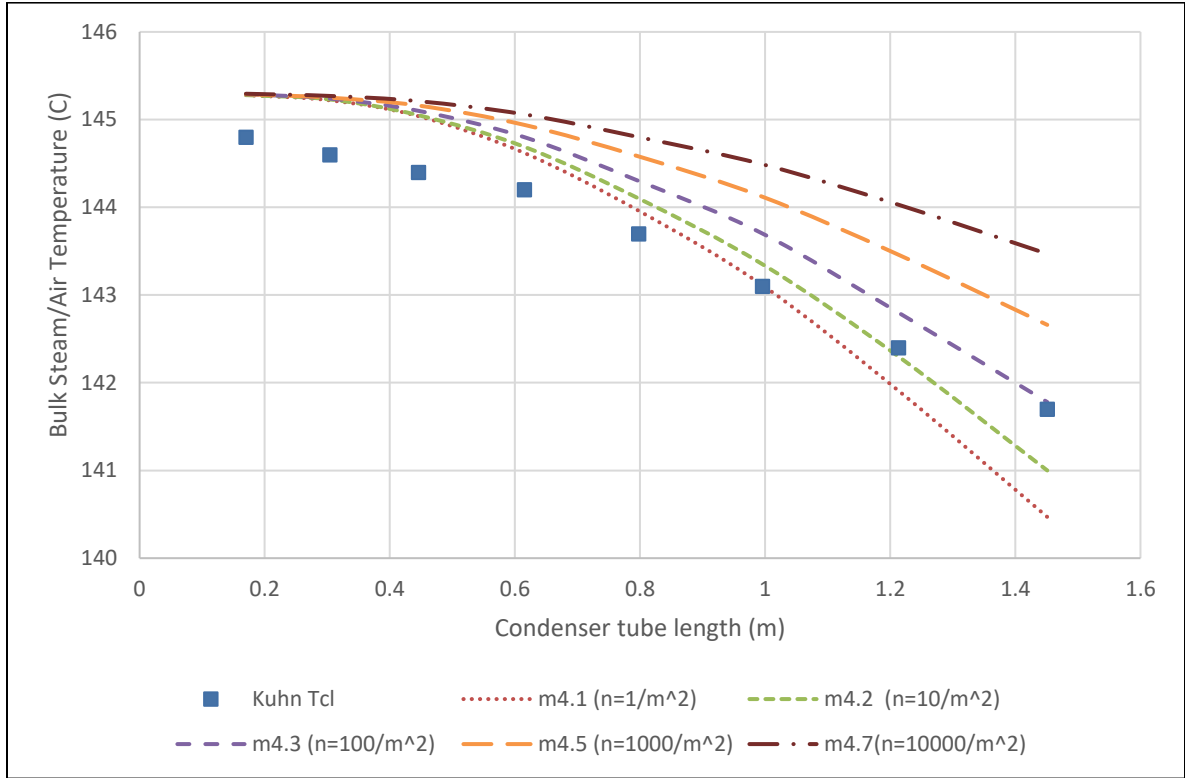
Figure 5.7 Droplet seed density variation study
