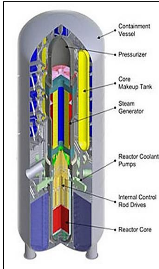
Figure 1.1 W-SMR [7]
