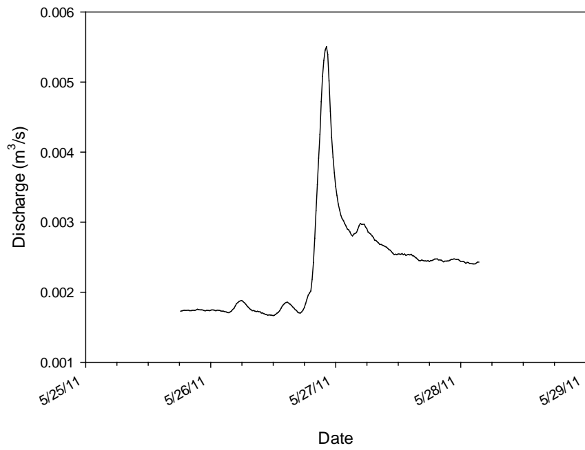
Figure D.15. Discharge from GC02 on May 25, 2011.
