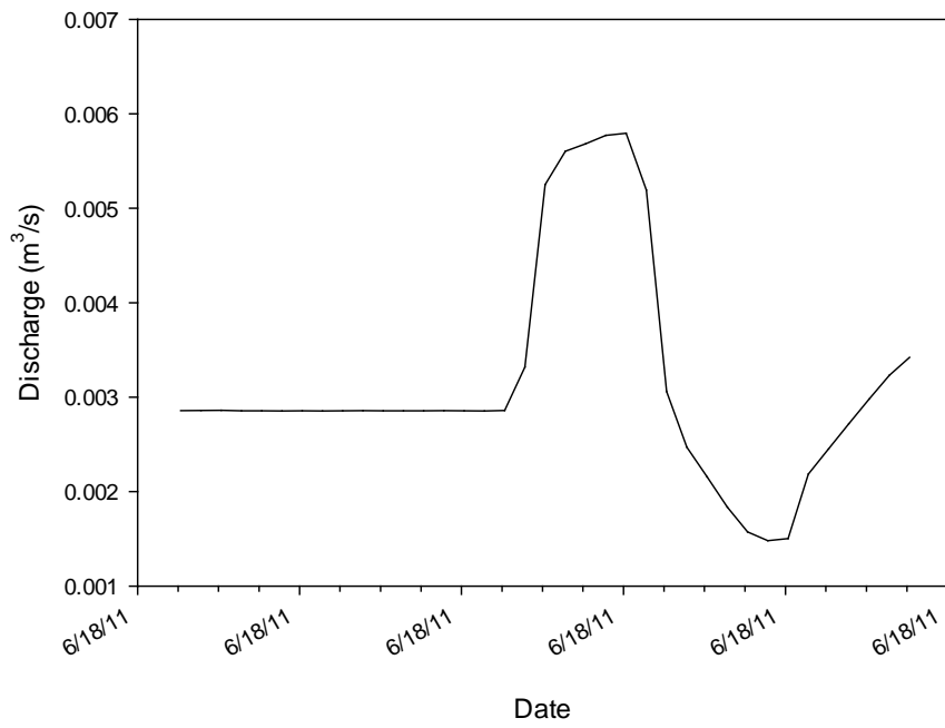
Figure E.23. Discharge from GC03 on June 17, 2011.
