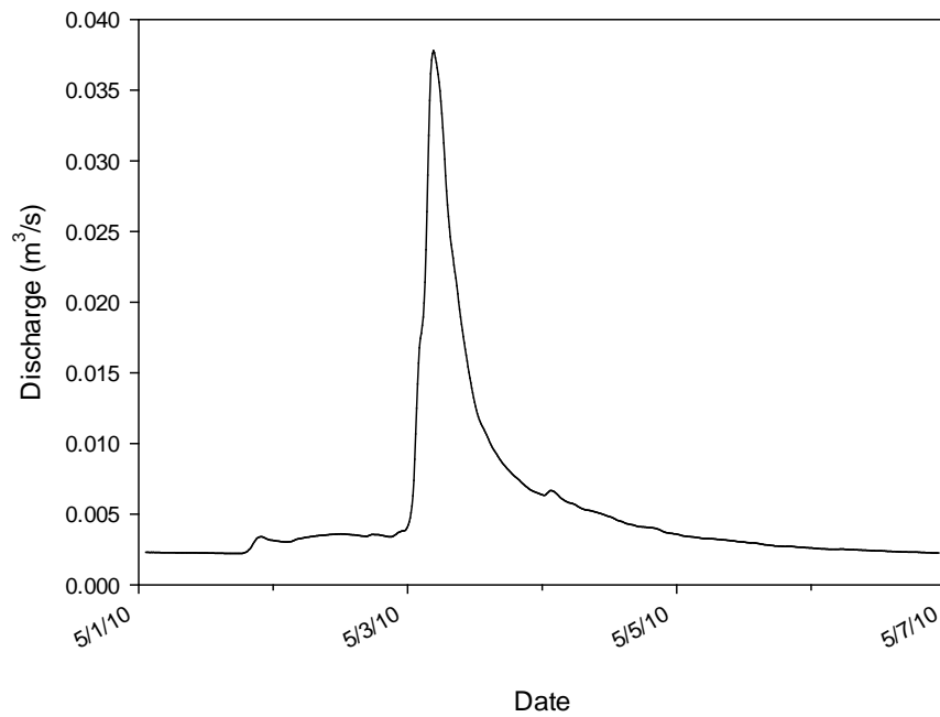
Figure C.4. Discharge from GC01 on May 1, 2010.
