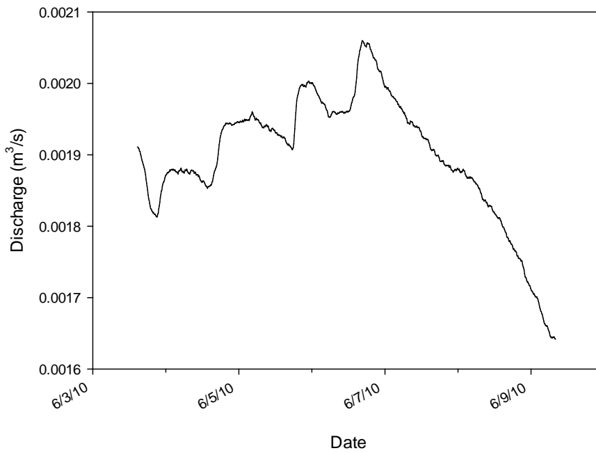
Figure C.6. Discharge from GC01 on June 4, 2010.
