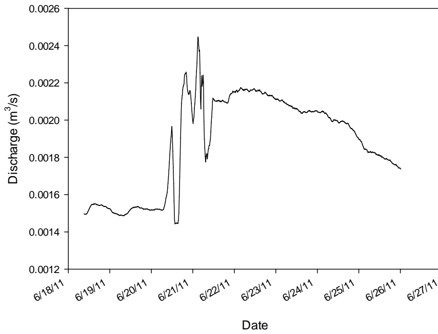
Figure C.15. Discharge from GC01 on June 18, 2011.
