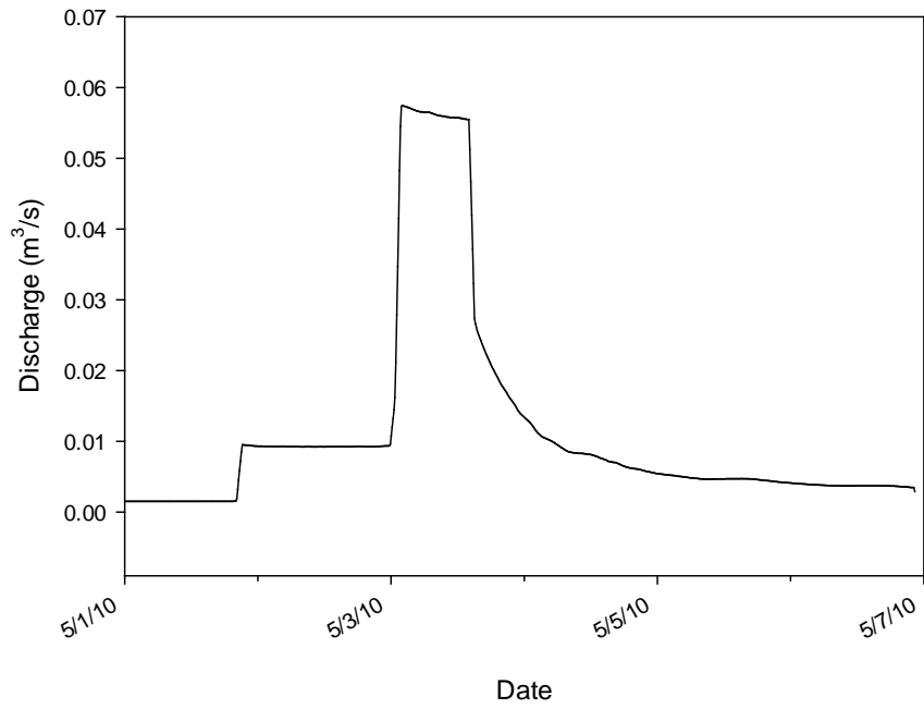
Figure D.3. Discharge from GC02 on May 1, 2010.
