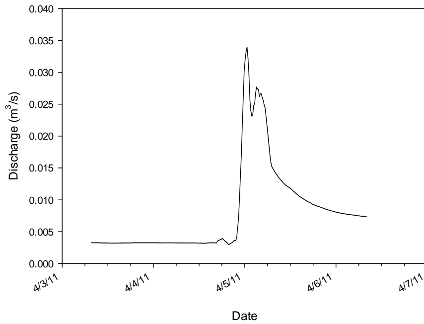
Figure E.13. Discharge from GC03 on April 2, 2011.
