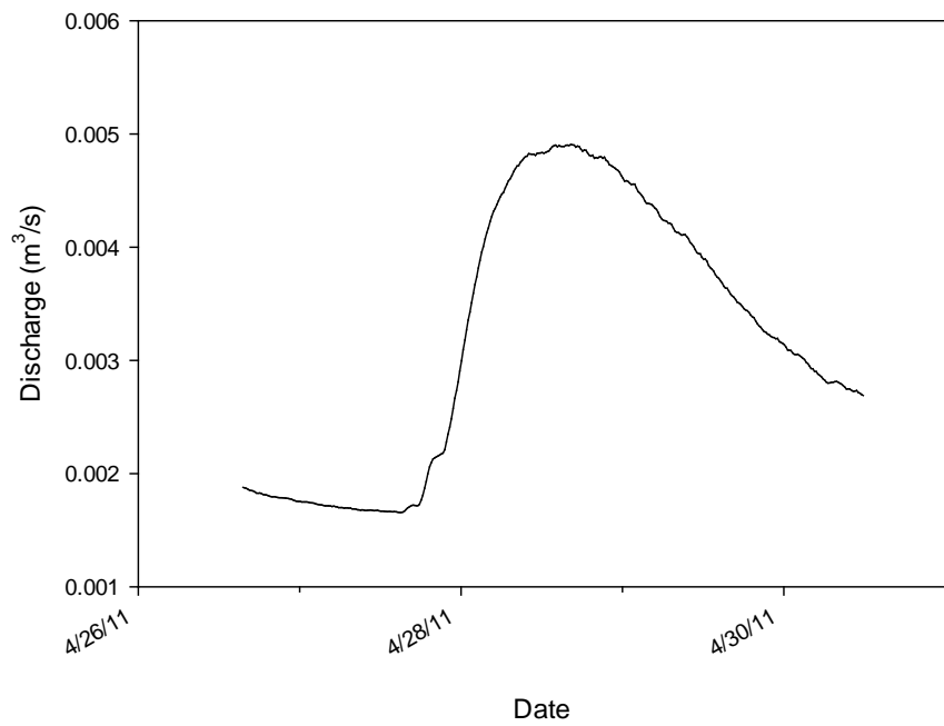
Figure C.12. Discharge from GC01 on April 26, 2011.
