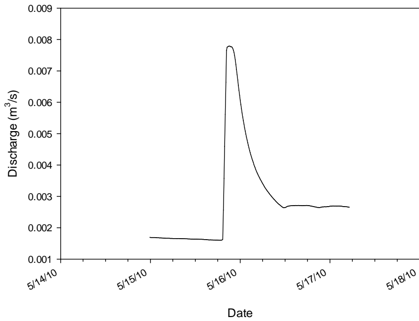
Figure D.4. Discharge from GC02 on May 14, 2010.
