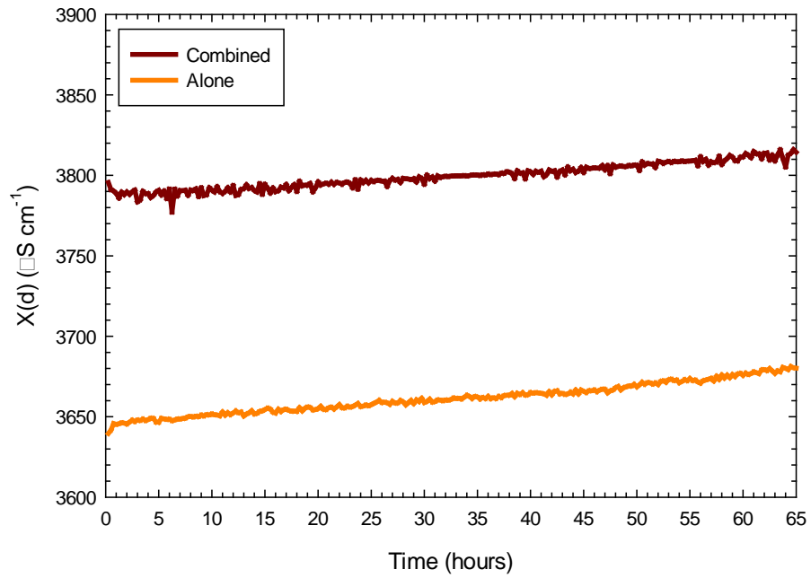
Figure 3.8 Laboratory Signal Interference Testing in EC 25°C Standard Waters
