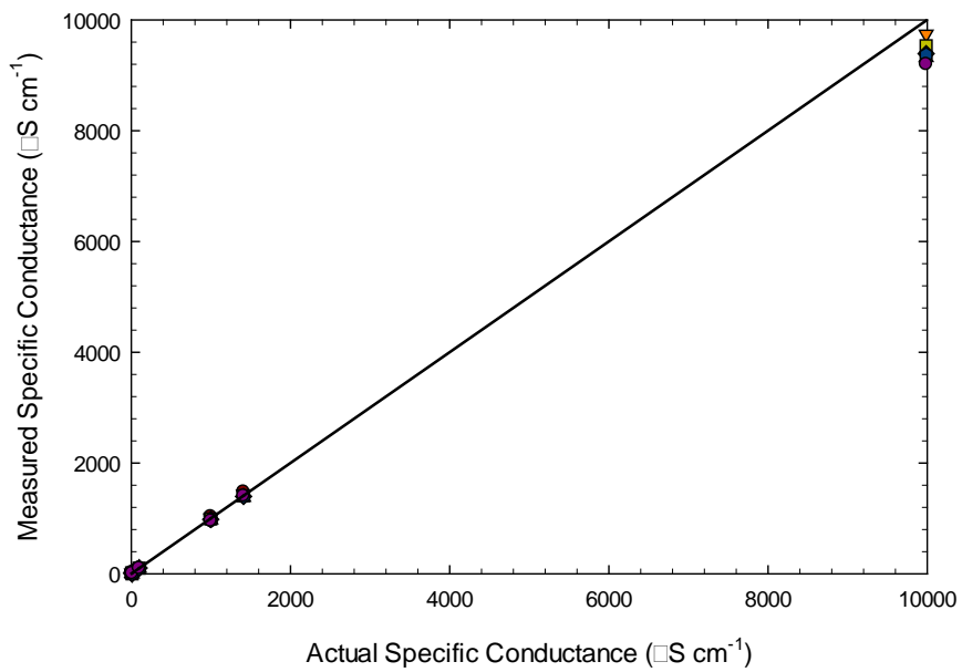
Figure 2.9 Actual EC 25°C plotted against measured EC 25°C of the Solinst sensor
