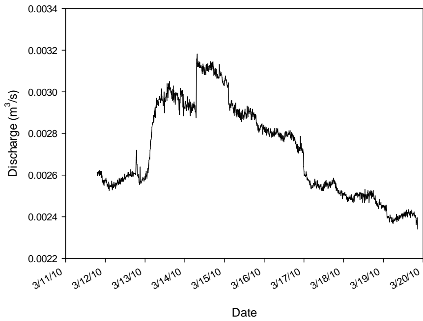
Figure C.1. Discharge from GC01 on March 12, 2010.
