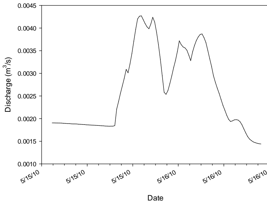
Figure C.5. Discharge from GC01 on May 14, 2010.
