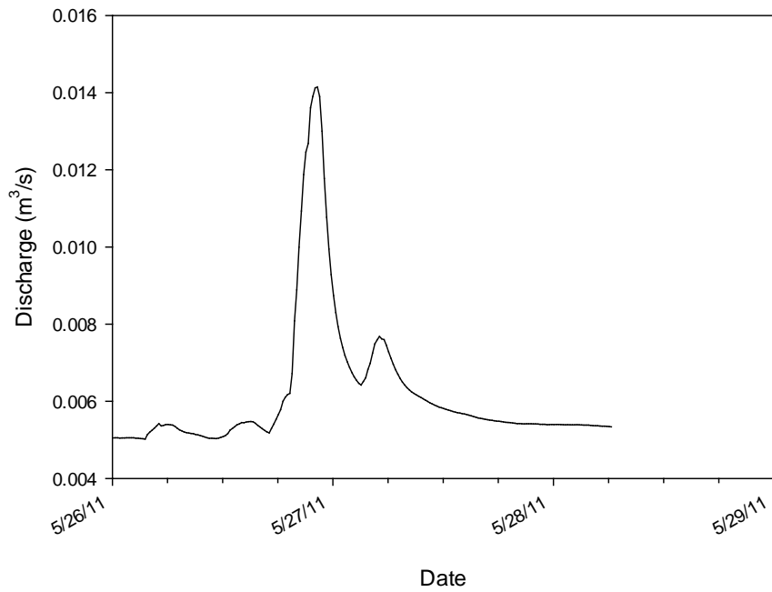
Figure E.22. Discharge from GC03 on May 25, 2011.
