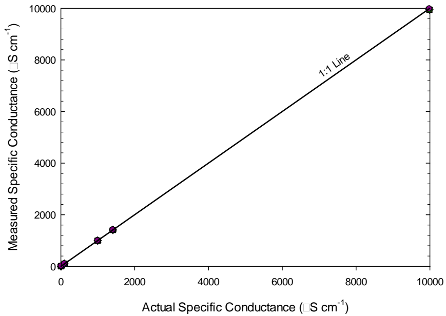
Figure 2.10 Actual EC 25°C plotted against measured EC 25°C of the HOBO sensor
