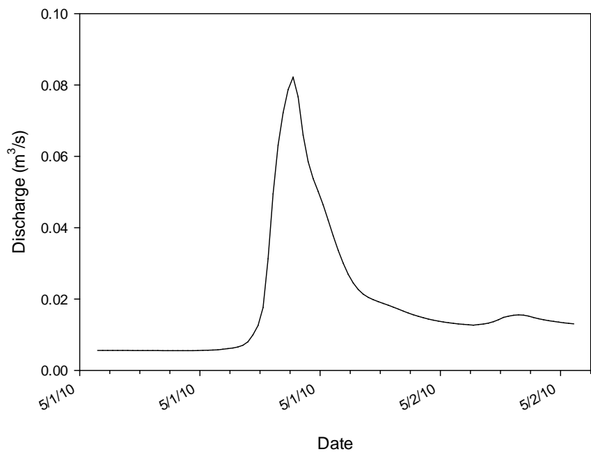
Figure E.4. Discharge from GC03 on May 1, 2010.
