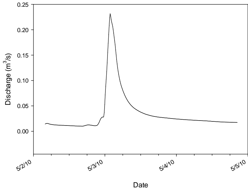
Figure E.5. Discharge from GC03 on May 2, 2010.
