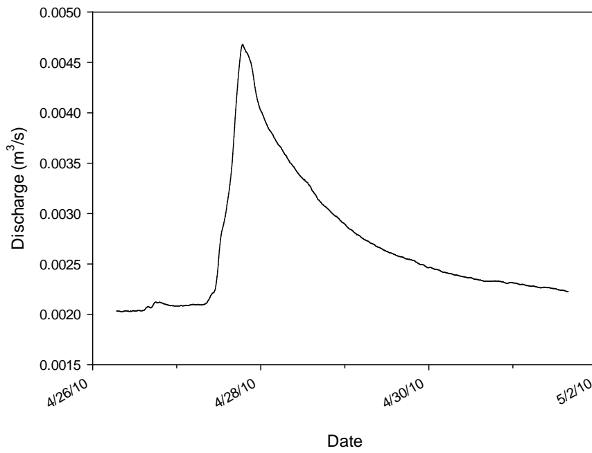
Figure C.3. Discharge from GC01 on April 27, 2010.
