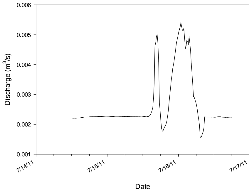
Figure E.26. Discharge from GC03 on July 14, 2011.
