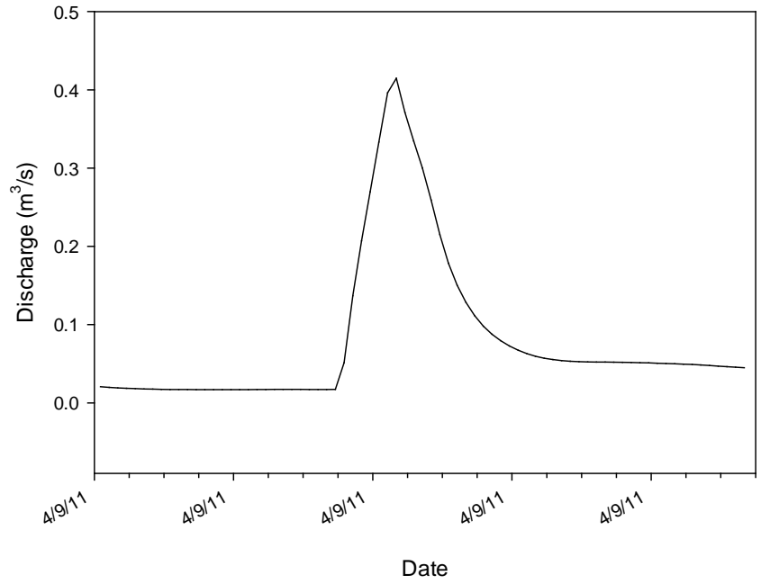
Figure F.13. Discharge from GC04 on April 8, 2011.
