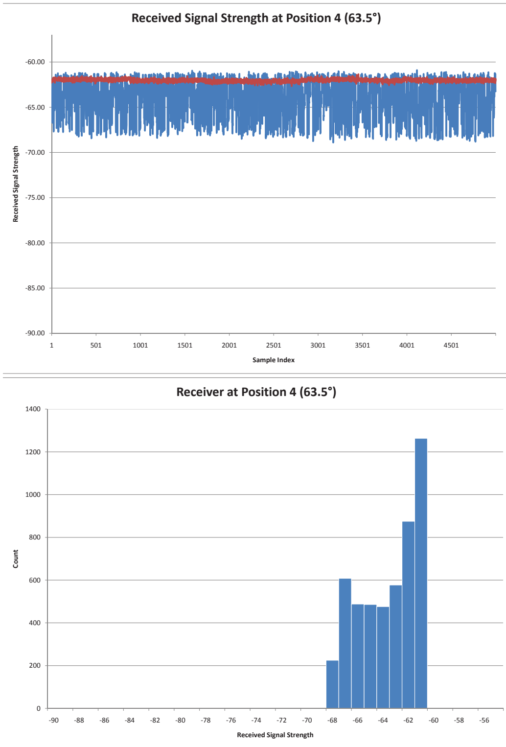
Figure 4.12: Received Signal at Position 4 (63.5°) of the Classroom. Top: Blue represents RSSI measurements using two-antenna phased array while red represents the RSSI measurements using a single antenna. Bottom: Histogram showing variation of the data samples collected for two-antenna phased array system
