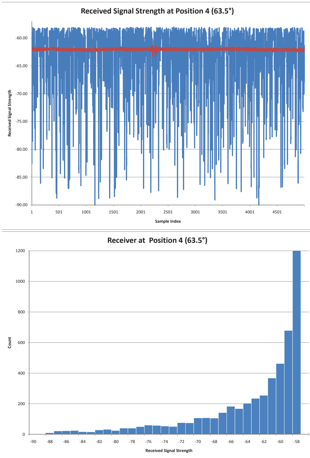
Figure 4.7: Received Signal at Position 4 (63.5°) of the Laboratory. Top: Blue represents RSSI measurements using two-antenna phased array while red represents the RSSI measurements using a single antenna. Bottom: Histogram showing variation of the data samples collected for two-antenna phased array system
