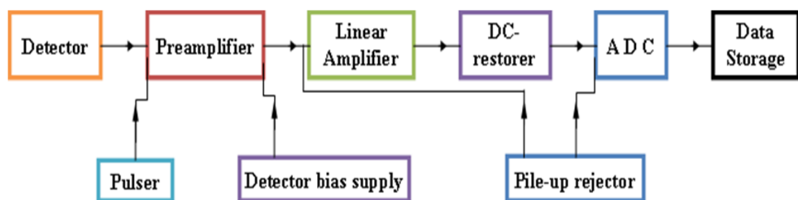
Figure 2.4. Schematic of Electronic System for Semiconductor Detector
