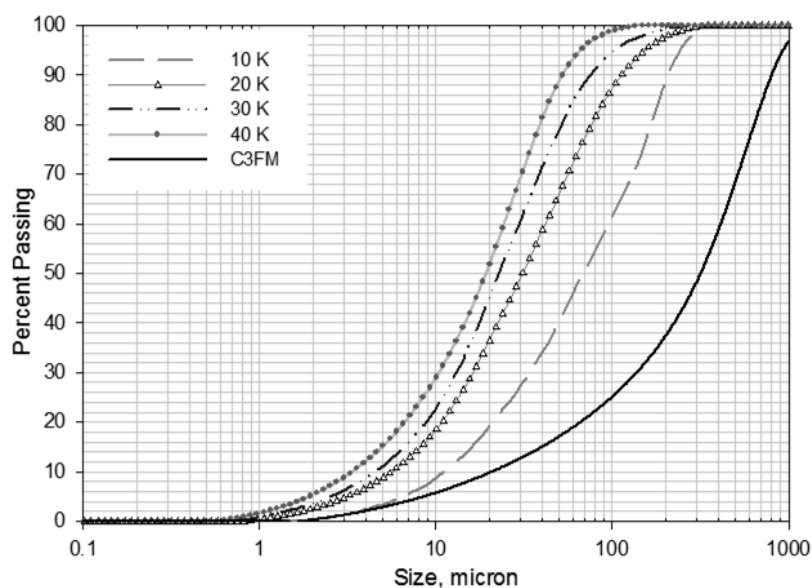
Figure 4.56. 98 mm Standoff Distance: CVUSCs of Products Obtained from C3FM Comminuted at Different Operational Pressures
