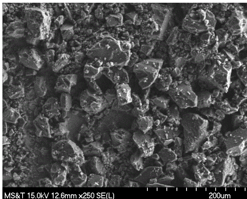
Figure 4.23. Morphological Properties of the Product Obtained from C2FM (10,000 psi Operational Pressure)
