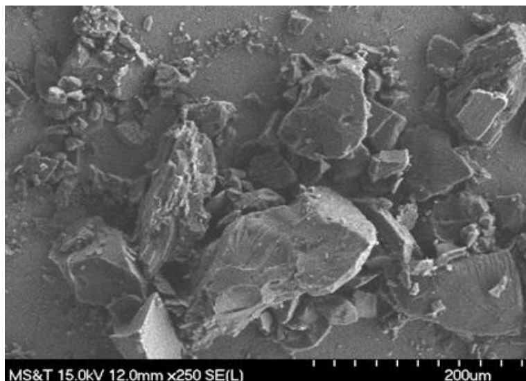
Figure 4.9. Morphological Properties of the Original Feed Material (C1FM)
