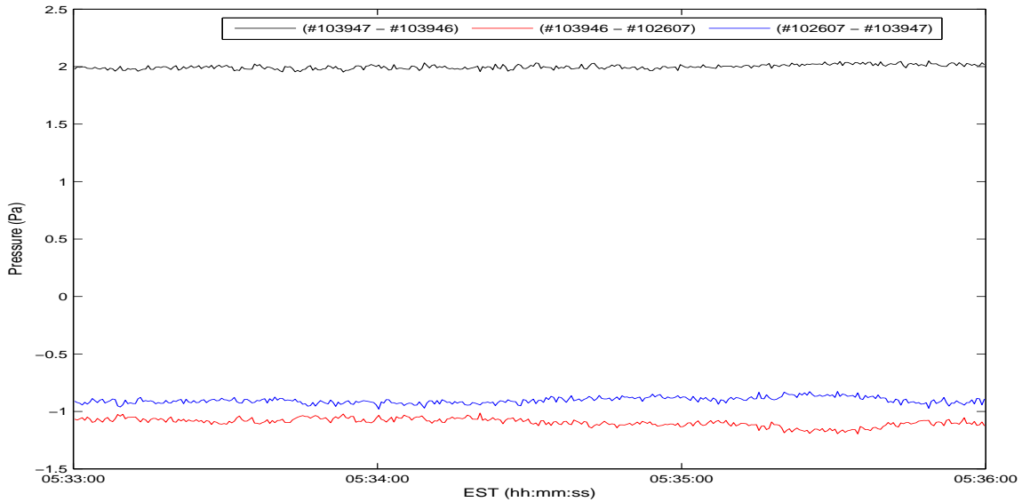
Figure 5.8. Time series of the difference between the three signals of figure 5.5. The mean values are 1.9980 Pa, -1.0946 Pa and -0.9034 Pa with standard deviations of 0.0193 Pa, 0.0348 Pa and 0.0270 Pa respectively.
