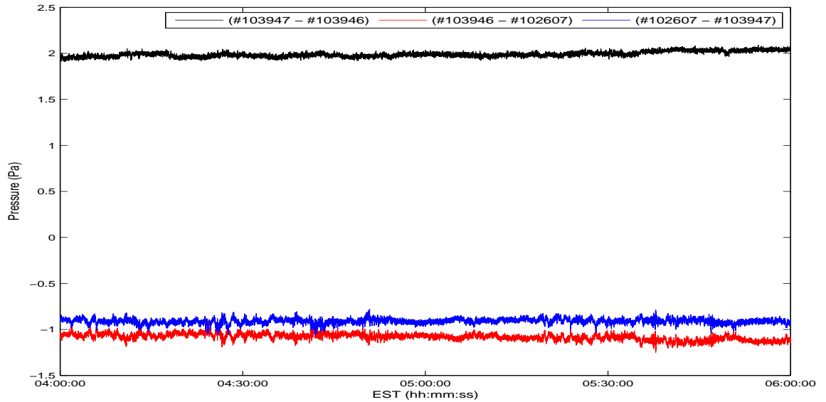
Figure 5.2. Time series of the difference between the three signals of figure 5.1: The mean values are 1.990 Pa, -1.0803 Pa and -0.9097 Pa with standard deviations of 0.0289 Pa, 0.0371 Pa and 0.0289 Pa respectively. When the barometer with DigiPort is involved, trends on the order of 1-3 min can be observed.
