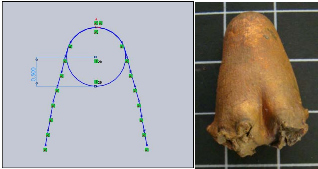
Figure 4.1: Projectile 3 and its cross section (inches).
