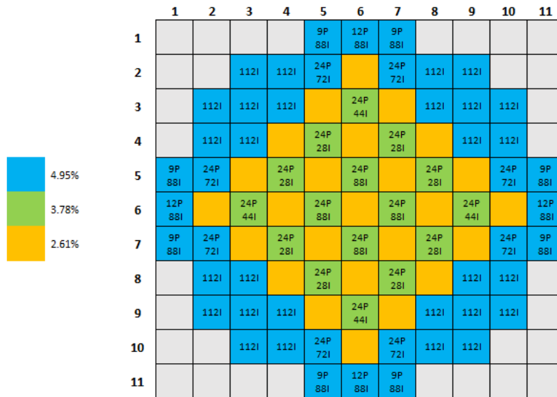
Figure 2.4. Proposed Core 3 Configuration
