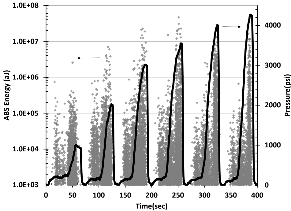
Figure 3.10: Pressure loading for internal damage to sample 13464-17-06-3 with recorded AE events
