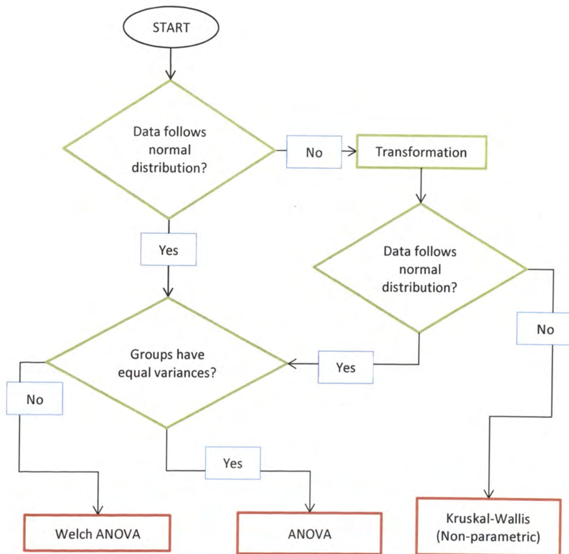
Figure 5-2 Algorithm of choosing an appropriate test of comparing the means (more than two groups)
