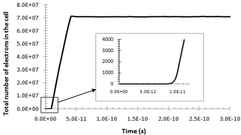
Figure 4.1. Total number of emitted electrons in the triode structure as a function of time. Grid voltage: 42V, anode voltage: 30kV, no focusing.
