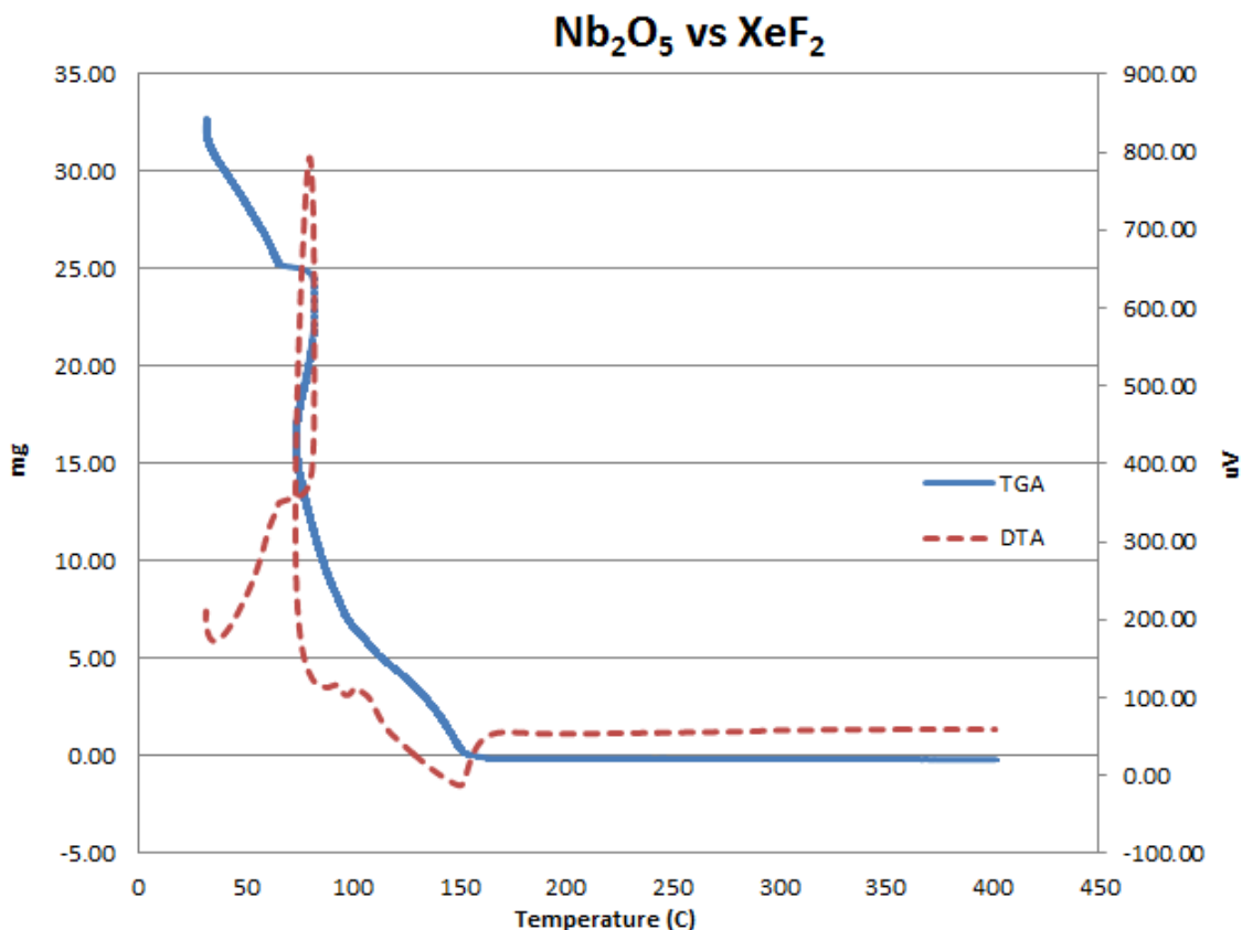
Figure 4.14. TG/DTA Data for Nb 2 O 5 /XeF 2
