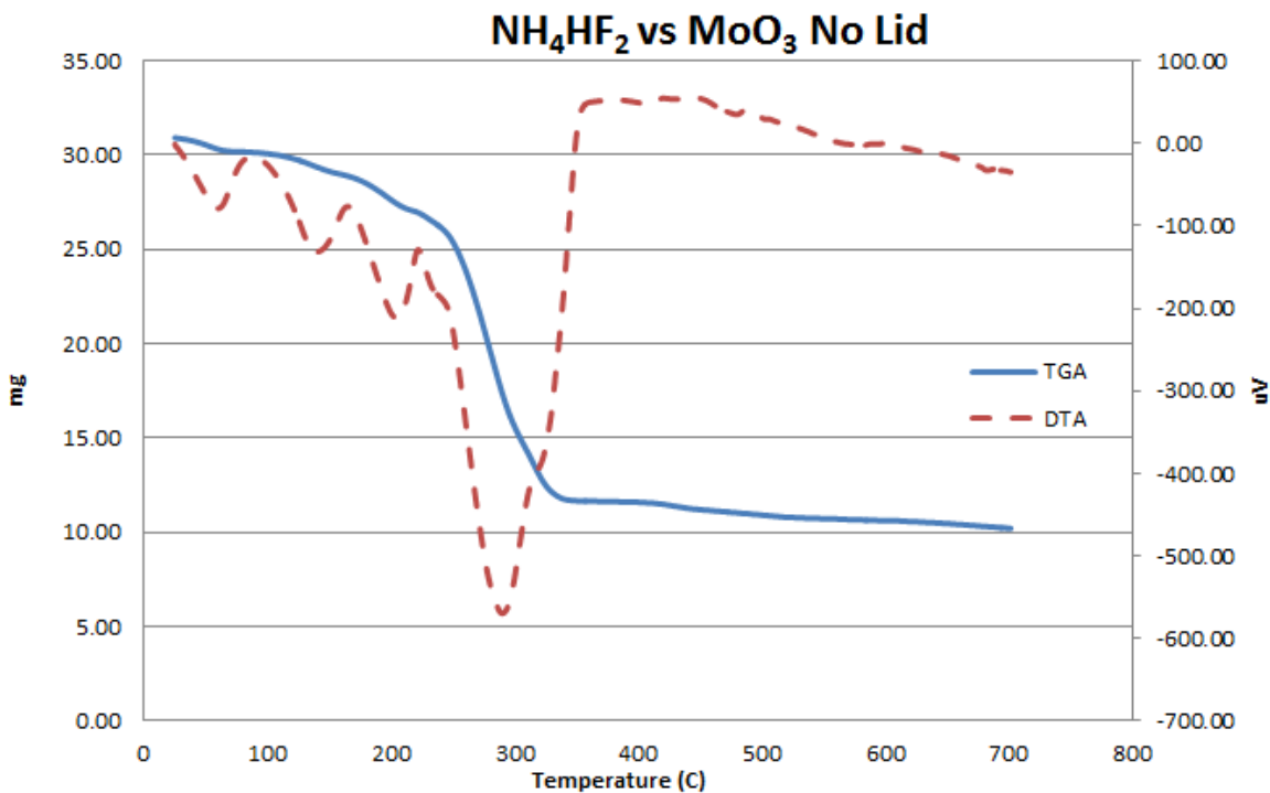
Figure 4.11. TG/DTA Data for MoO 3 /NH 4 HF 2 No Lid
