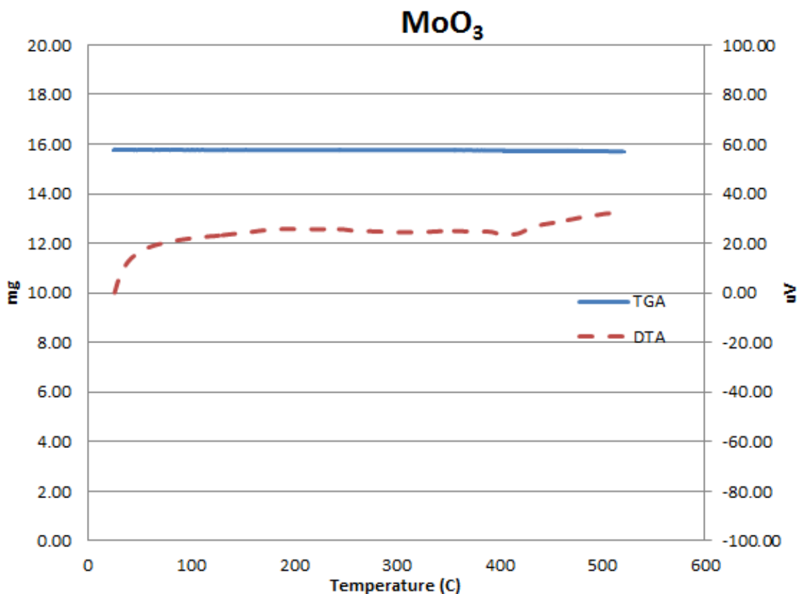
Figure 4.9. TG/DTA Data for MoO 3
