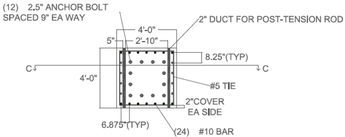
Figure 3.21 - Cross Section of Concrete Block (A-A)
