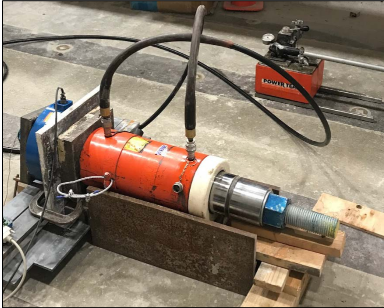
Figure 3.27 - Individual Calibration of Anchor Bolts
