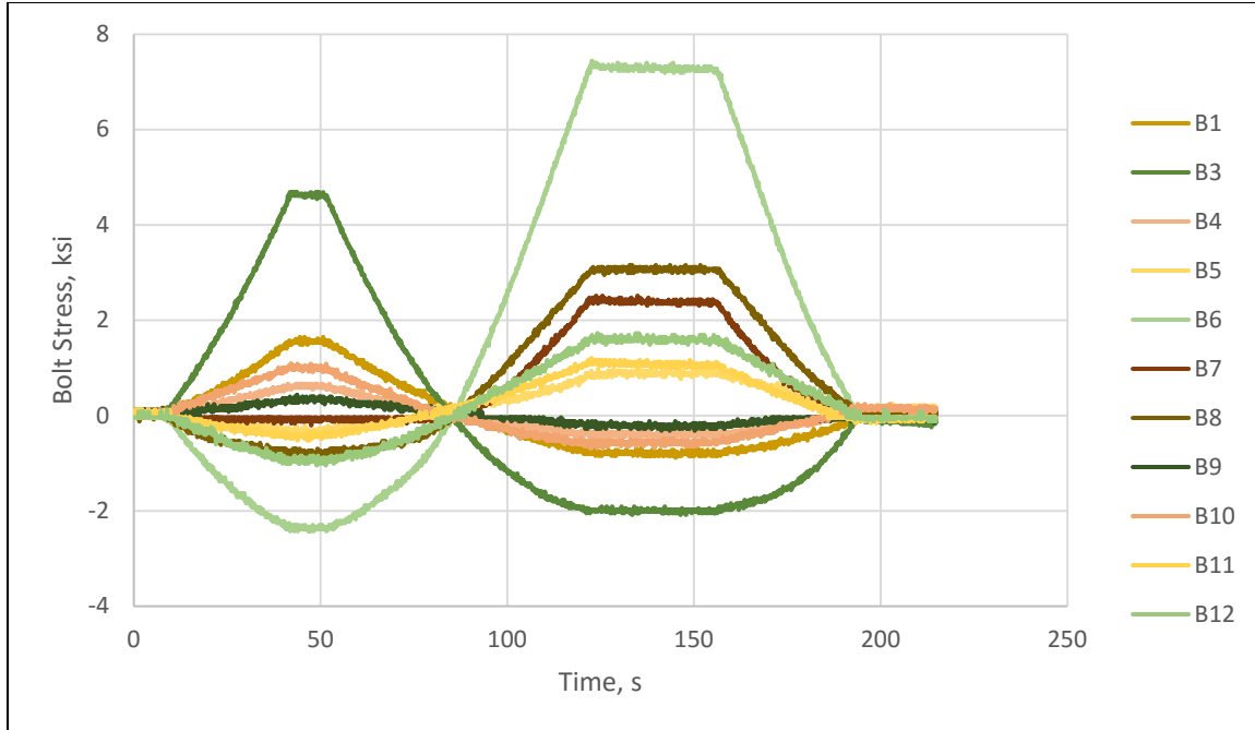
Figure 3.44 - Time vs. Bolt Stress
