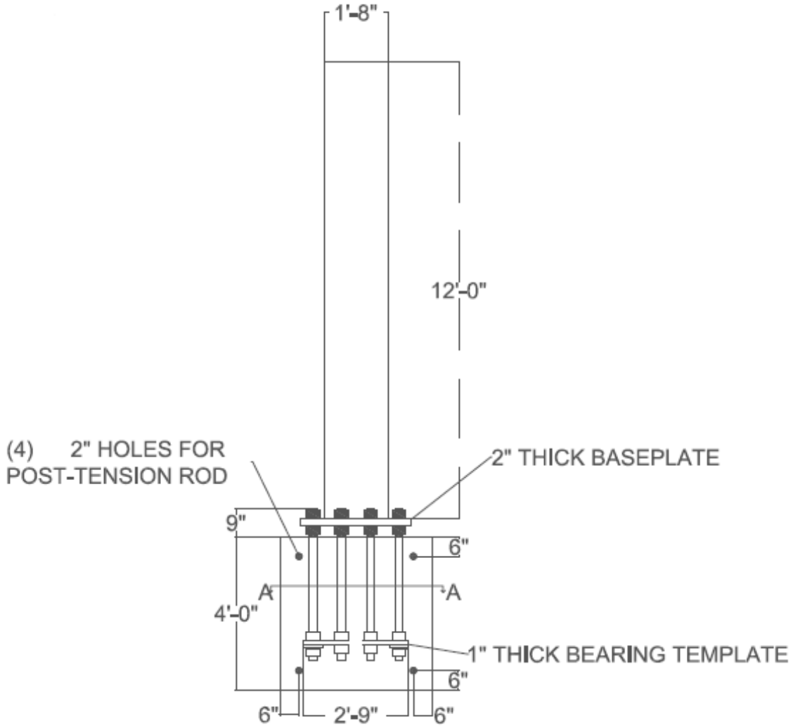
Figure 3.20 - Top View of Lab Specimen
