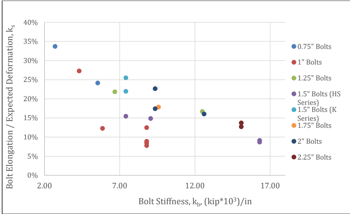
Figure 2.36 - Bolt Stiffness vs. k_s
