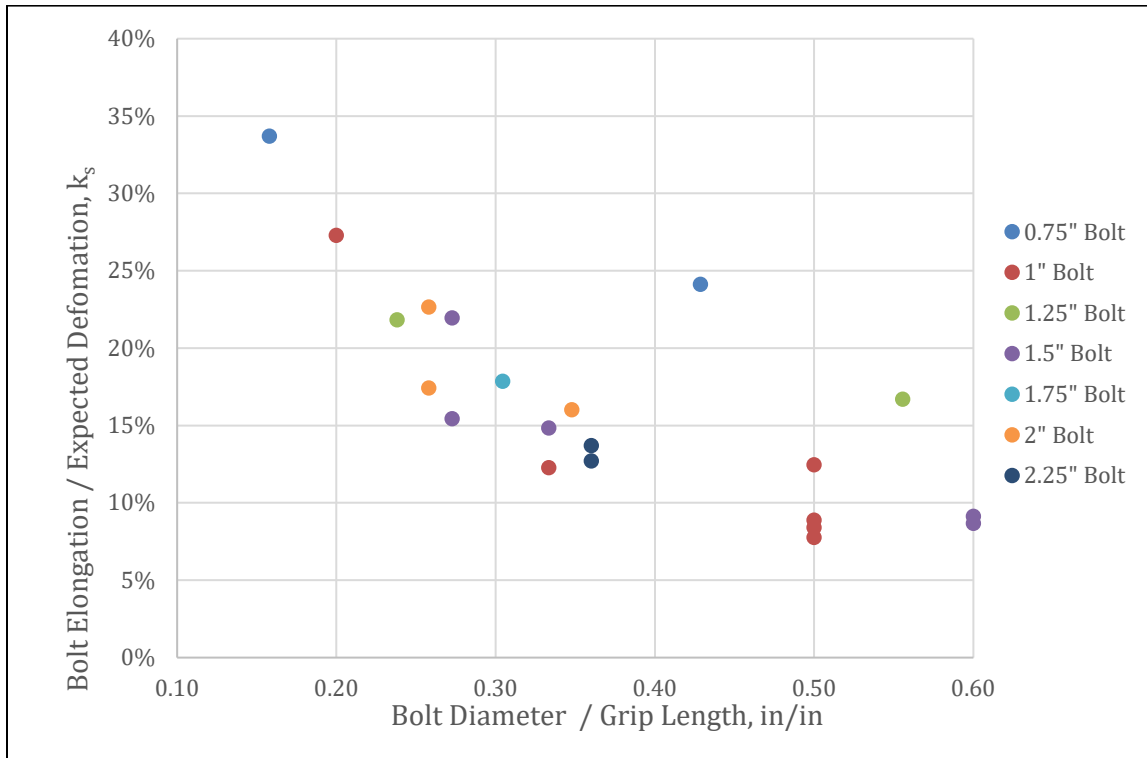
Figure 2.37 - Bolt Diameter / Grip Length vs. k_s
