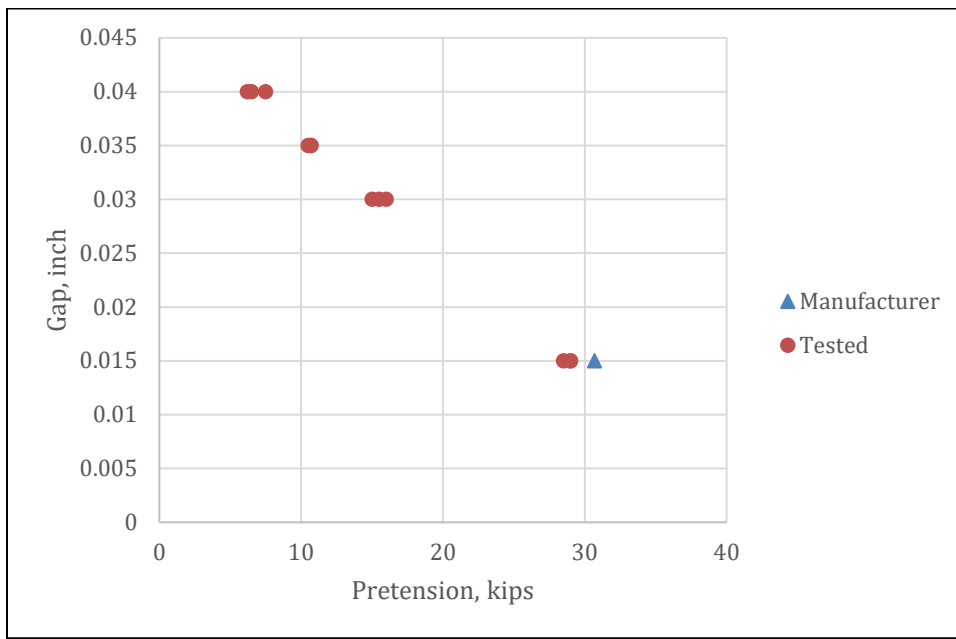
Figure 2.38 - 0.75" A325 DTI
