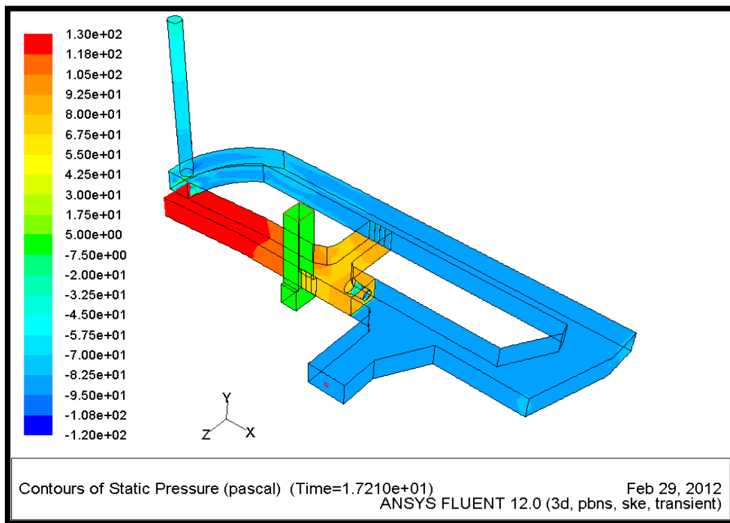
Figure 8.10. Pressure distribution contours across the domain
