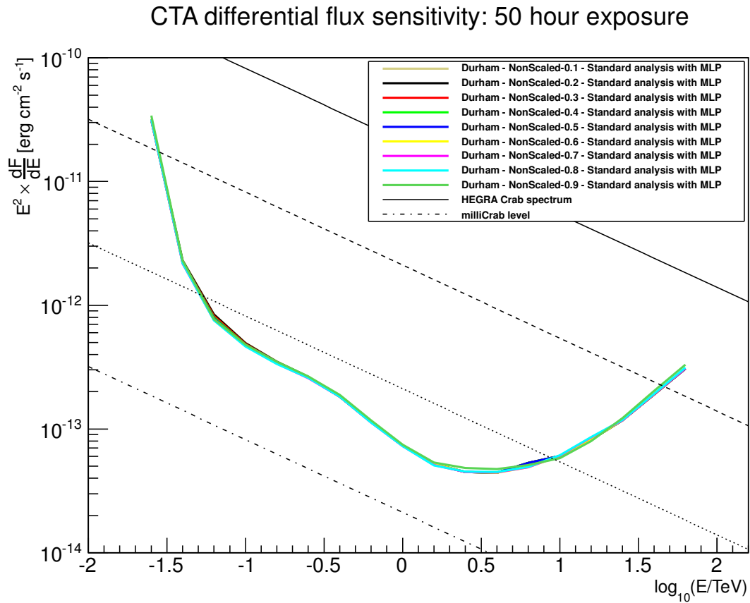
Figure 3.48: Differential sensitivity as a function of energy for Subarray-I calculated using different values for the fixed TMVA::MLP cut parameter. The derived values for the differential sensitivity do not appear to be sensitive to the cut value chosen for this particular method of deriving the TMVA::MLP cut parameter. However the concerns highlighted in Section 3.4 regarding the fixed cut method should be taken into consideration.
