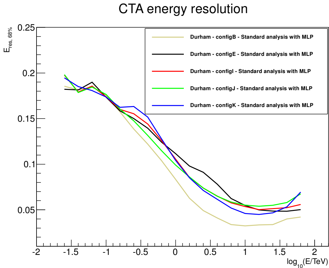
Figure 3.23: Derived energy resolution as a function of energy for all analysed subarrays. Subarray-B appears to be the best performing subarray for energy resolution. This is because Subarray-B is relatively compact and comprised of 5 LSTs and 37 MSTs, meaning it has a comparatively large light collecting area with lower triggering thresholds, optimising the subarray for nearby events. The other subarrays all have a similar energy resolution performance.
