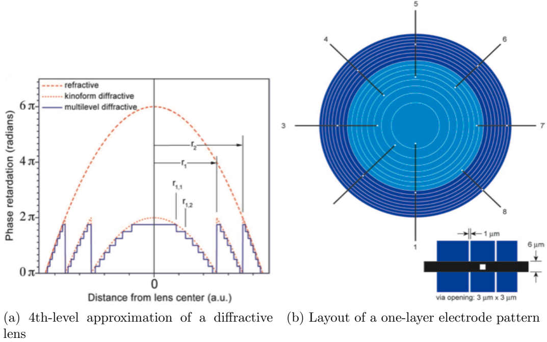
Figure 2.7: Designs for an LC diffractive lens from [41].
