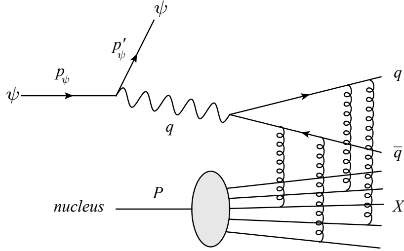
Fig. 5.5.: The dipole scattering with occurs via gluon exchange between the dipole and quarks in the nucleus.
