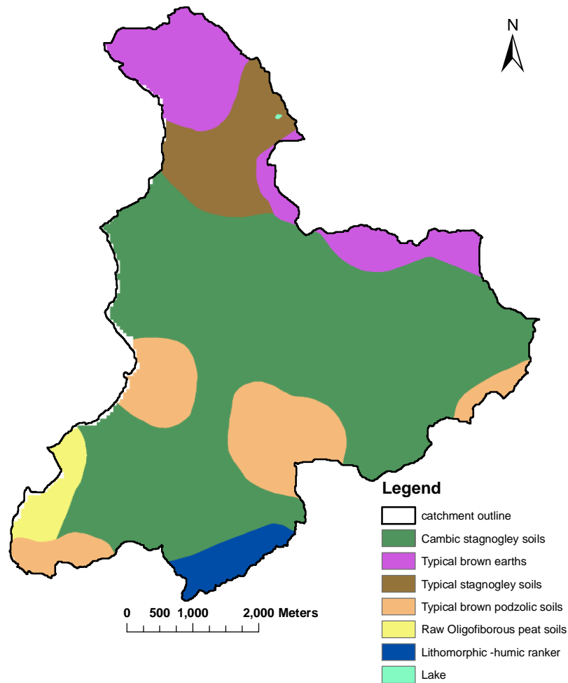
Figure 2.9 Soils of the Dacre Beck catchment (data from NATMAP 5000 provided by LandIS, Cranfield University)
