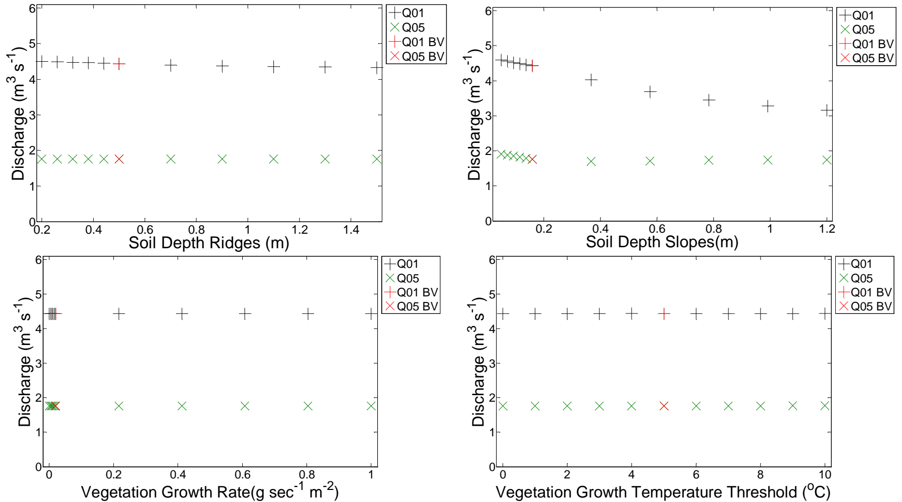
Figure A3.2 High flows sensitivity response graphs
