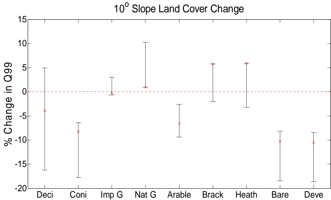
Figure 5.5 10° slope scenario impacts on Q99
