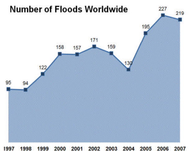
Figure 1.1 Numbers of floods worldwide 1997-2007 data from (Black and King, 2009).
