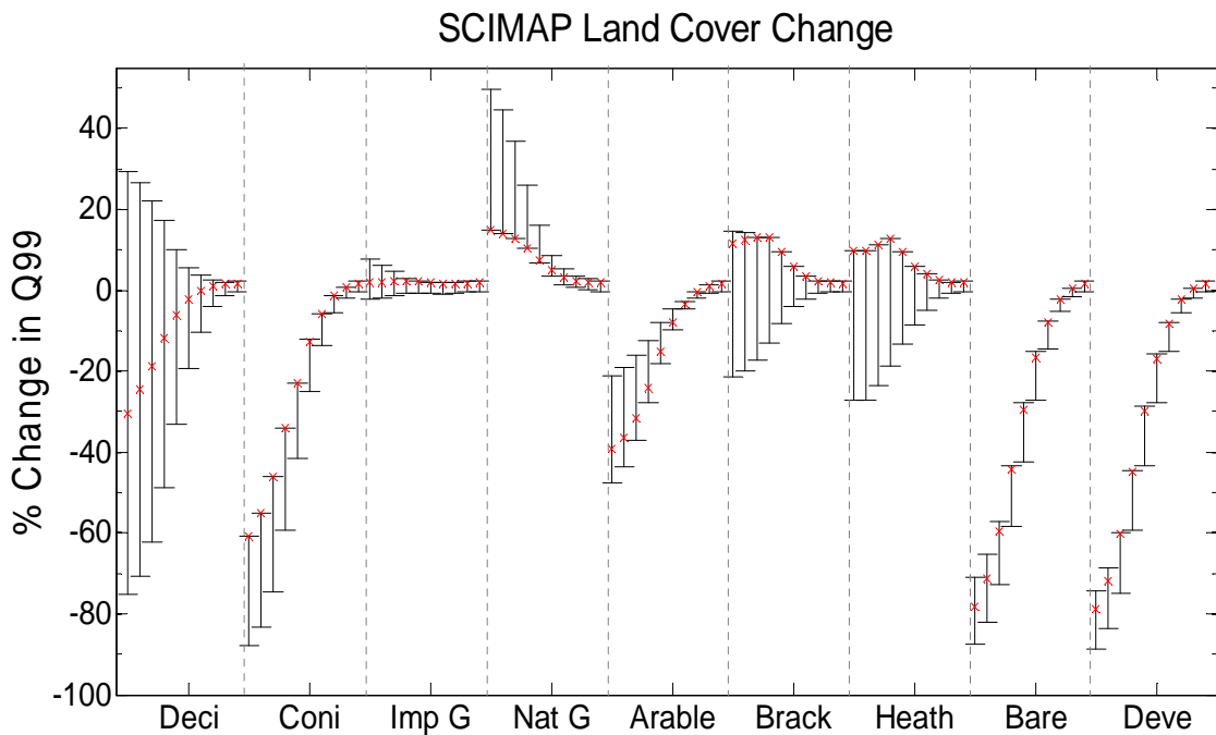
Figure 5.13 Overall impact of SCIMAP scenarios on Q99
