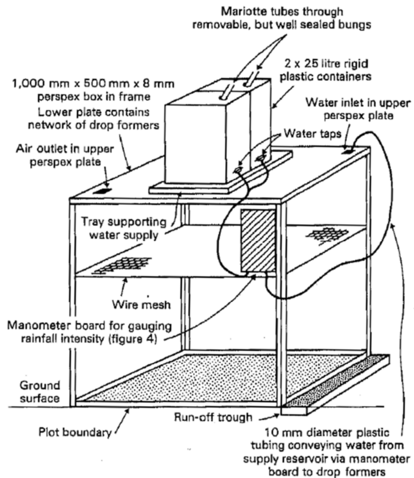
Figure 3.8 'Drip-type' Rainfall Simulator (Bowyer-Boyer and Burt, 1989).
