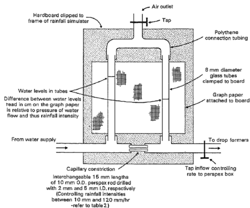
Figure 3.9 Manometer for the control of rainfall intensity (Bowyer-Bower and Burt, 1989)
