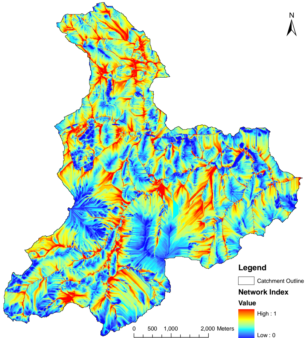
Figure 5.11 SCIMAP Network Index Map
