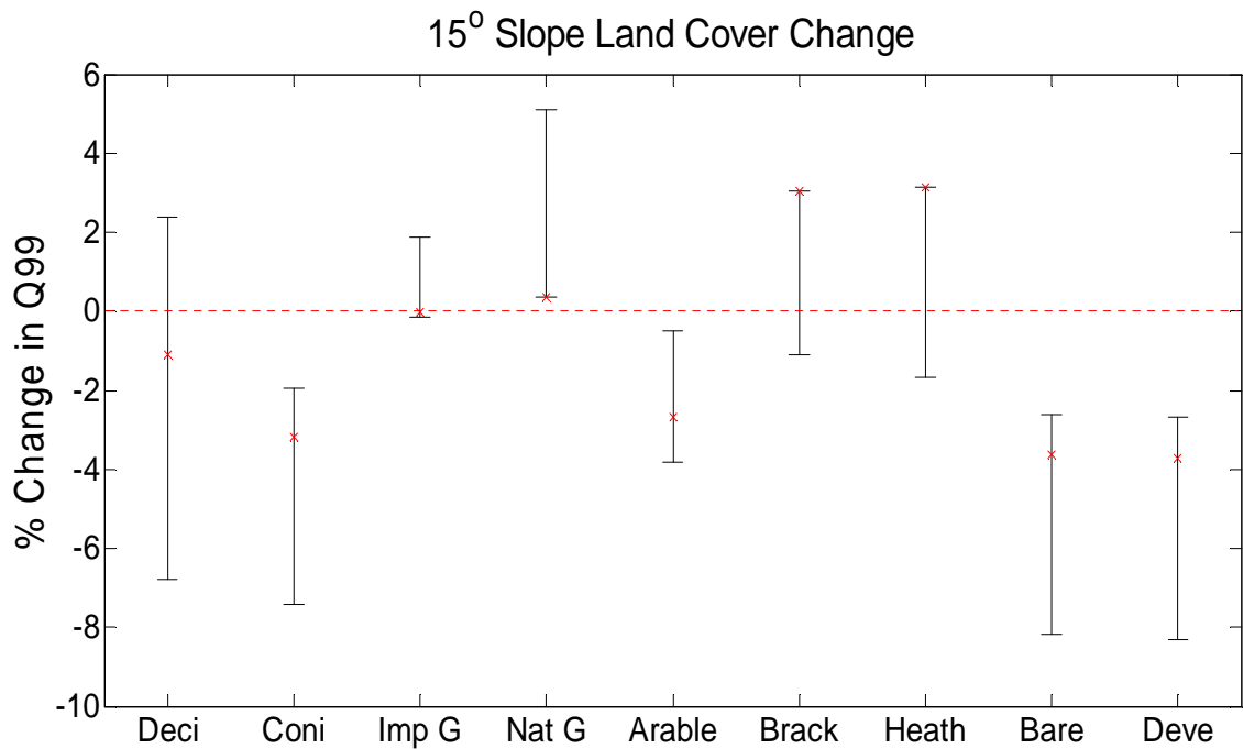
Figure 5.6 15° slope scenario impacts on Q99
