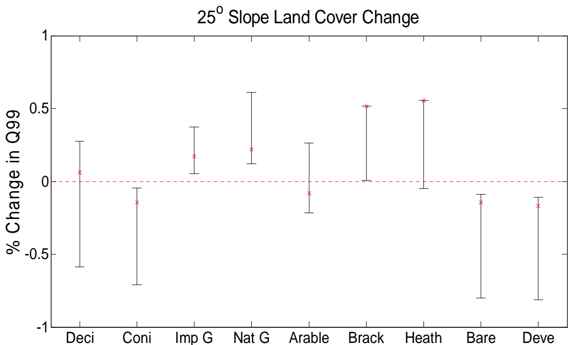
Figure 5.8 25° slope scenario impacts on Q99
