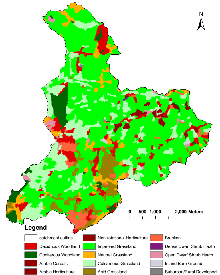
Figure 2.10 Land Cover Map of the Dacre Beck catchment (Land Cover Map 2000, Centre for Ecology and Hydrology)
