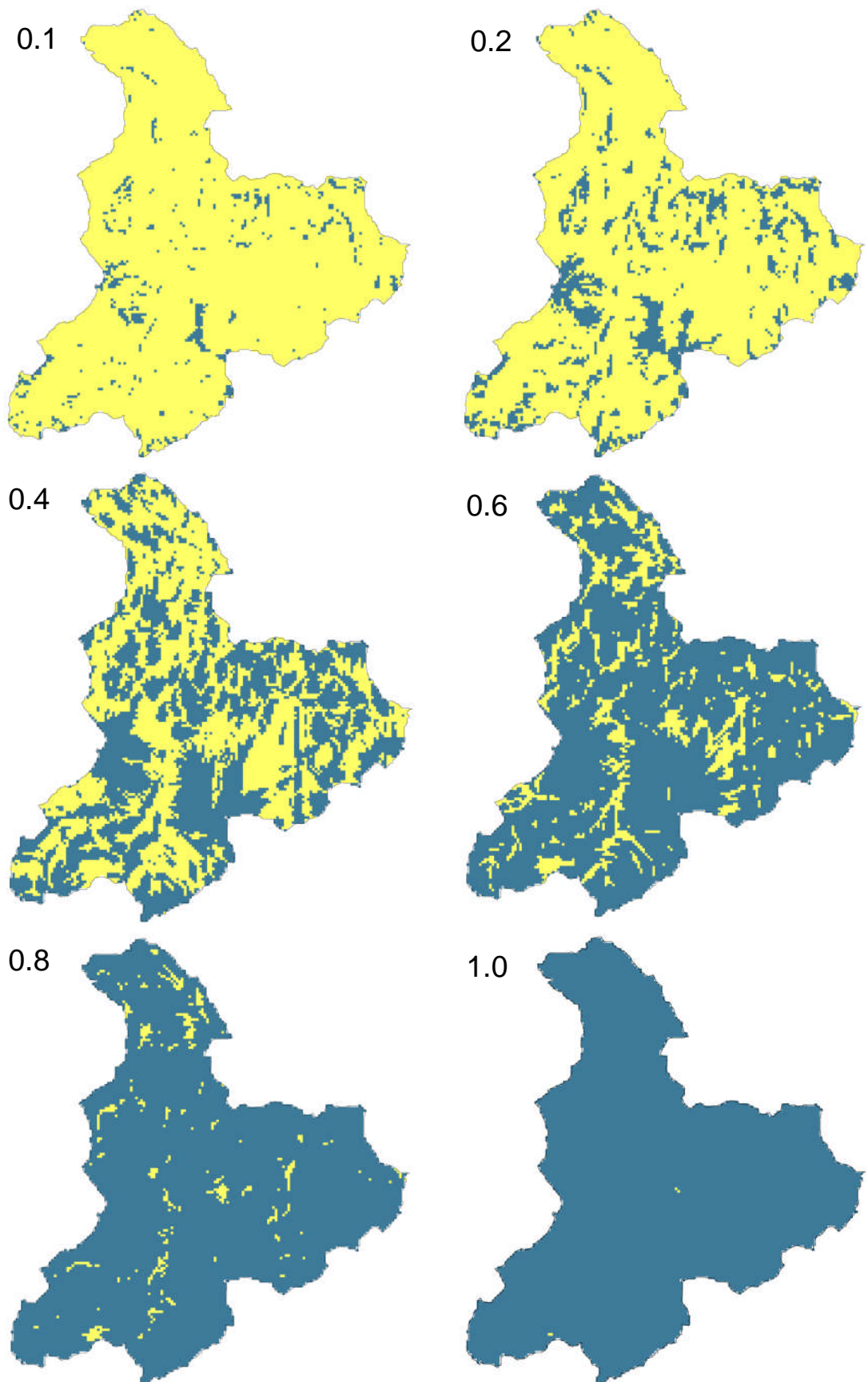
Figure 5.12 Area covered by the SCIMAP land cover scenarios: blue indicates land to be changed, yellow indicates land to remain as in the LCM2000.
