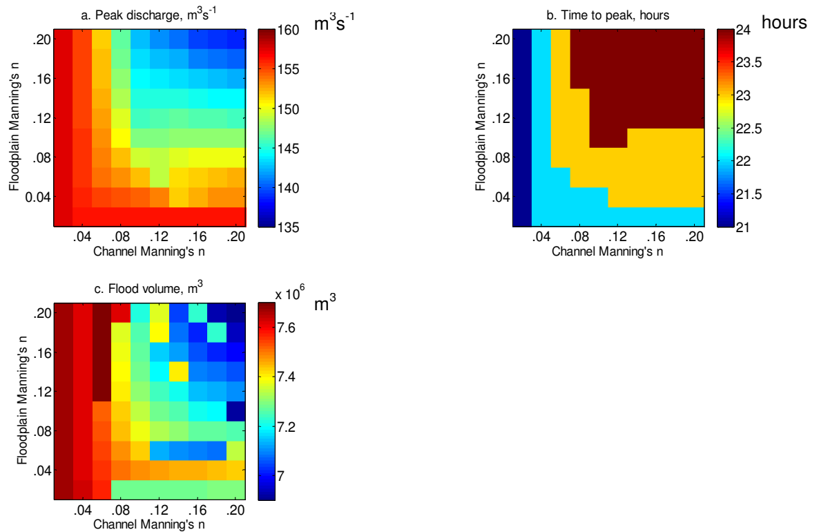
Figure 6.5 Summary statistics of HEC-RAS hydrograph sensitivity to variation in channel and floodplain Manning's n : (a) Peak discharge ( m^3 s^{-1} ), (b) Time to peak (hours after start of simulation) and (c) Overbank flood volume ( m^3 ). Values are given by the colour bar on the right of each plot.
