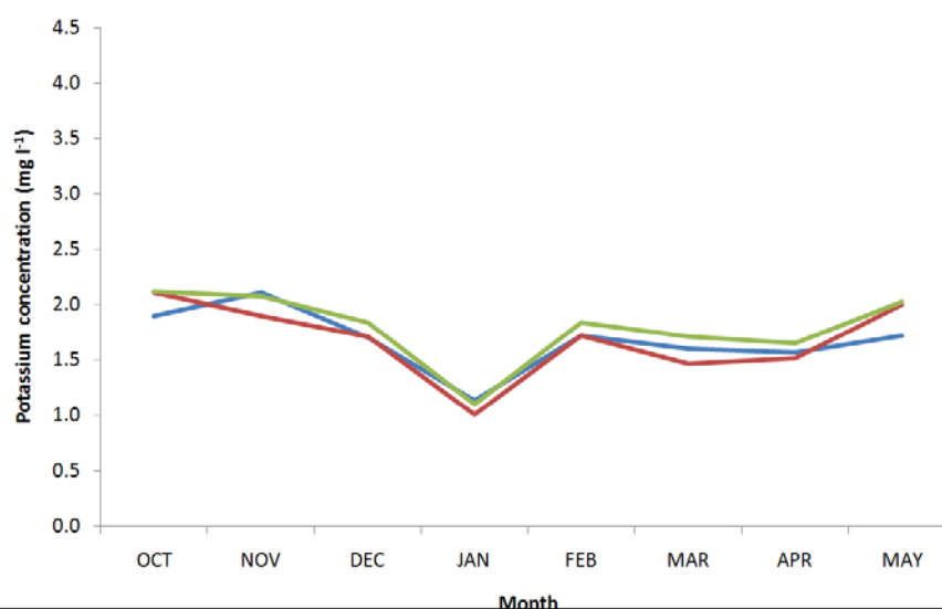
Figure 5.12: Monthly potassium concentrations at Lealholm; Grosmont; and catchment scale (monthly average)
