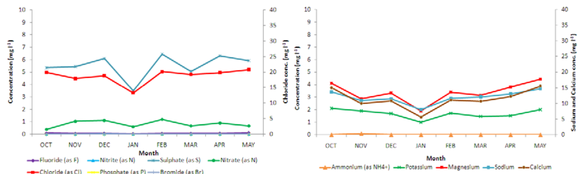
Figure 5.1: Temporal variation in anions (left) and cations (right) over the sampling period (Oct-May) at sites on the Esk at a. Danby Moors Centre; b. Castleton; c. Danby Road Bridge and; d. Lealholm
