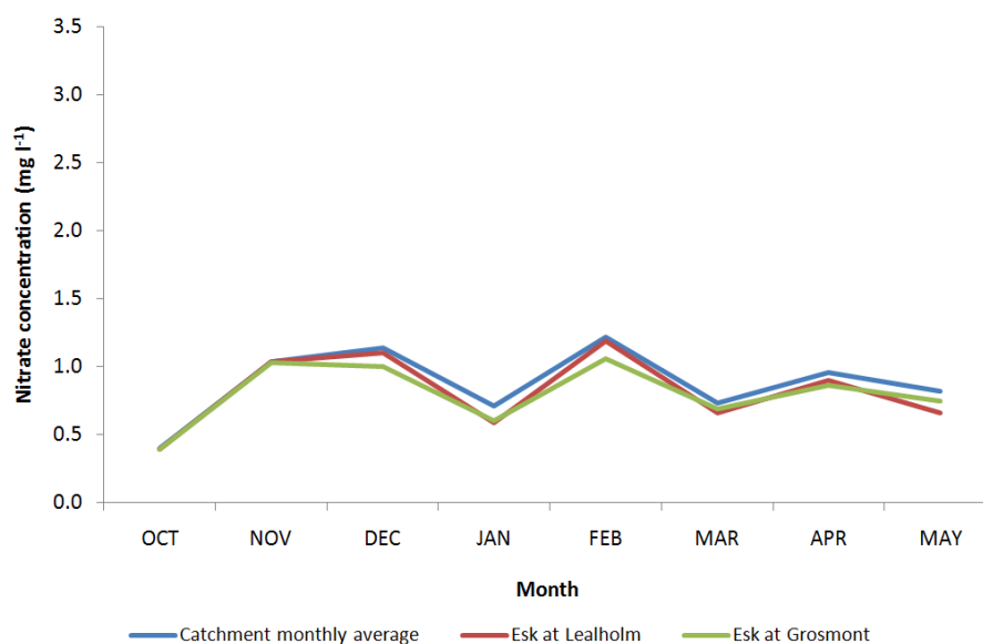
Figure 5.14: Monthly nitrate concentrations at Lealholm; Grosmont; and catchment scale (monthly average)
