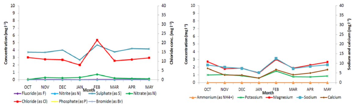
Figure 5.2 (part 1): Temporal variation in anions (left) and cations (right) over the sampling period (Oct- May) at sites on the Esk tributaries at a. Commondale Beck (upstream) and; b. Hob Hole
