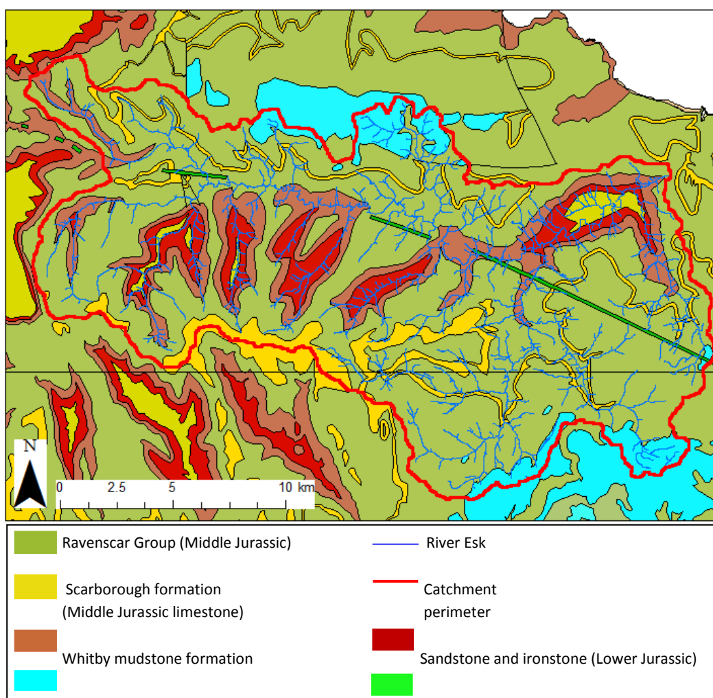
Figure 3.2a: Bedrock geologies in the Esk catchment and the surrounding region
