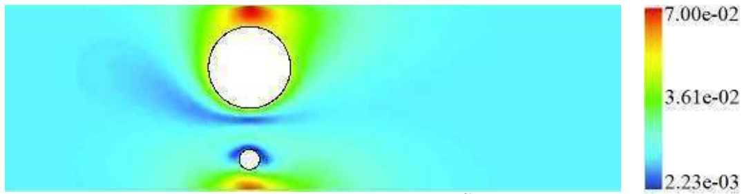
Velocity contours of counter-rotating cylinders at \tilde{S} = 0.5
