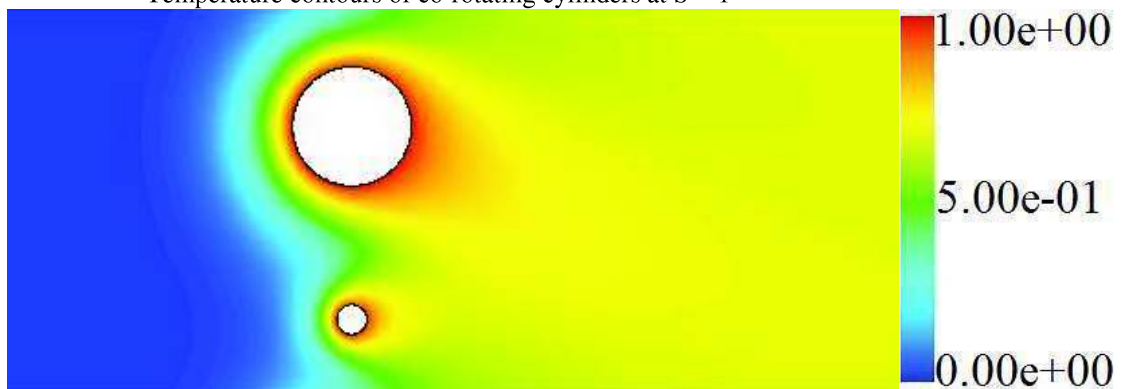
Temperature contours of counter-rotating cylinders at \tilde{S} = 1
