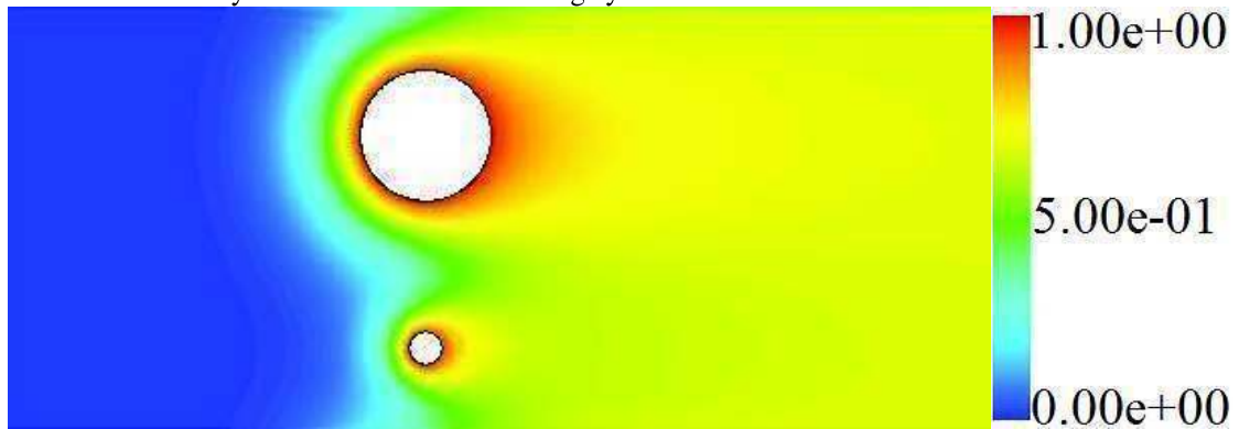
Temperature contours of stationary cylinders at \tilde{S} = 1
