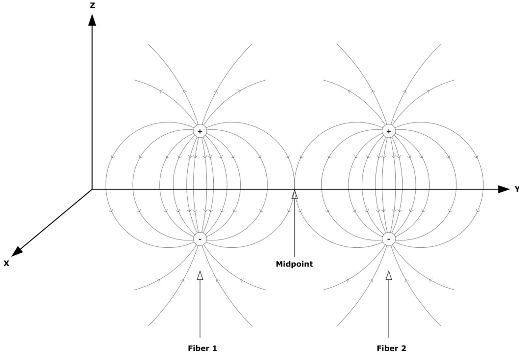
Figure 2.6: We choose the midpoint between two nanofibers to calculate the total electric field.
