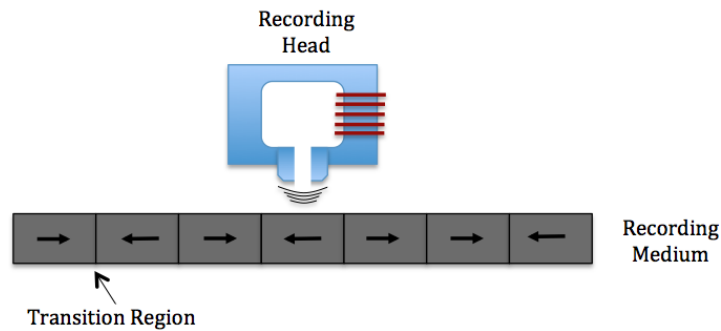
Figure 1.9 Longitudinal recording
