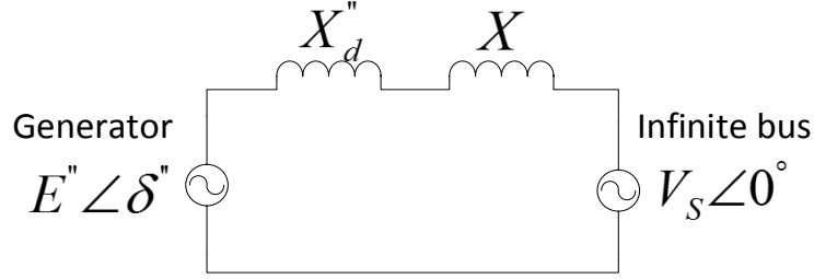
Figure 2.3 One-machine-infinite-bus system
