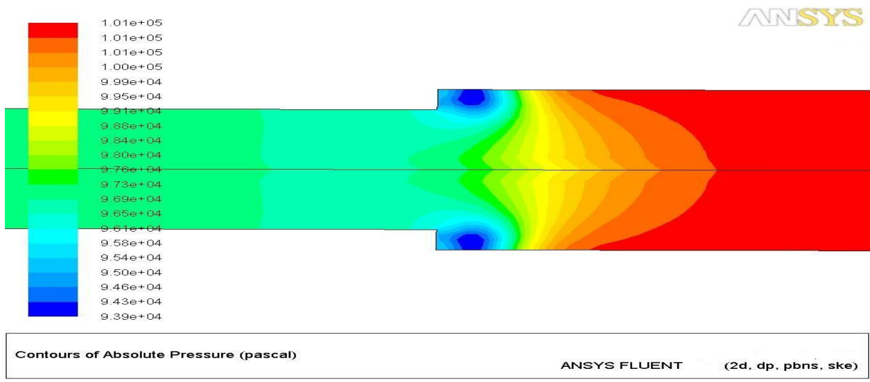
Fig 5.4: Contours of absolute pressure in pipe
