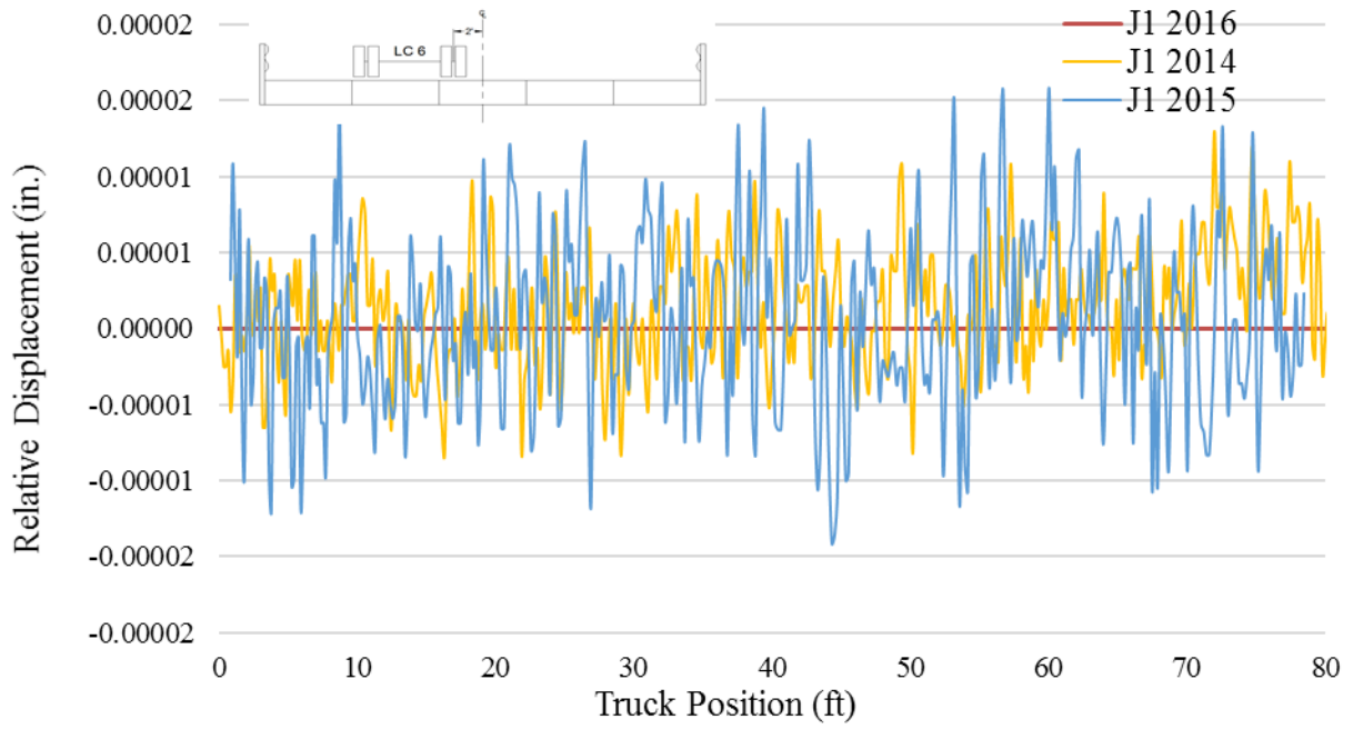
Figure 36. History of relative displacement at J1 (LC-6)
