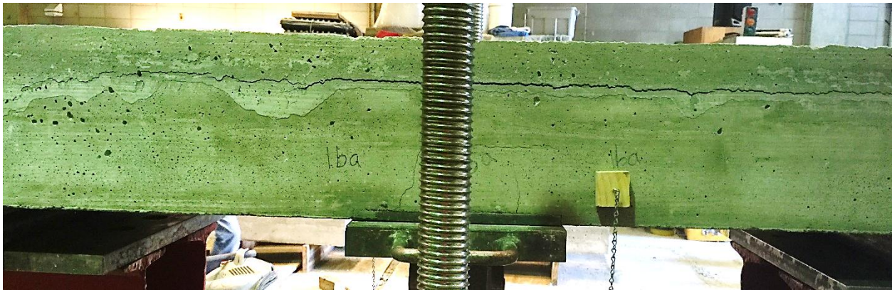
Figure 86. Case 1 positive bending flexural test specimen failure at concrete bond interface
