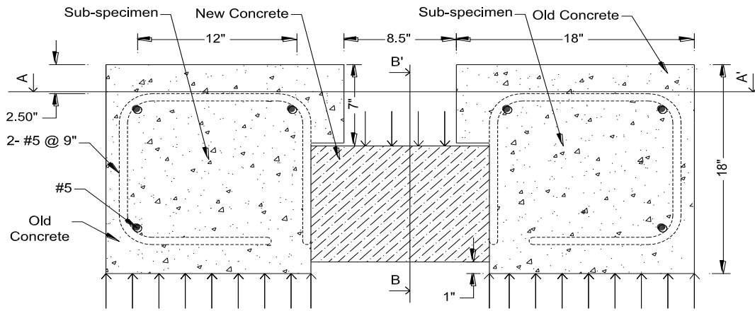
a) SECTIONAL SIDE VIEW
