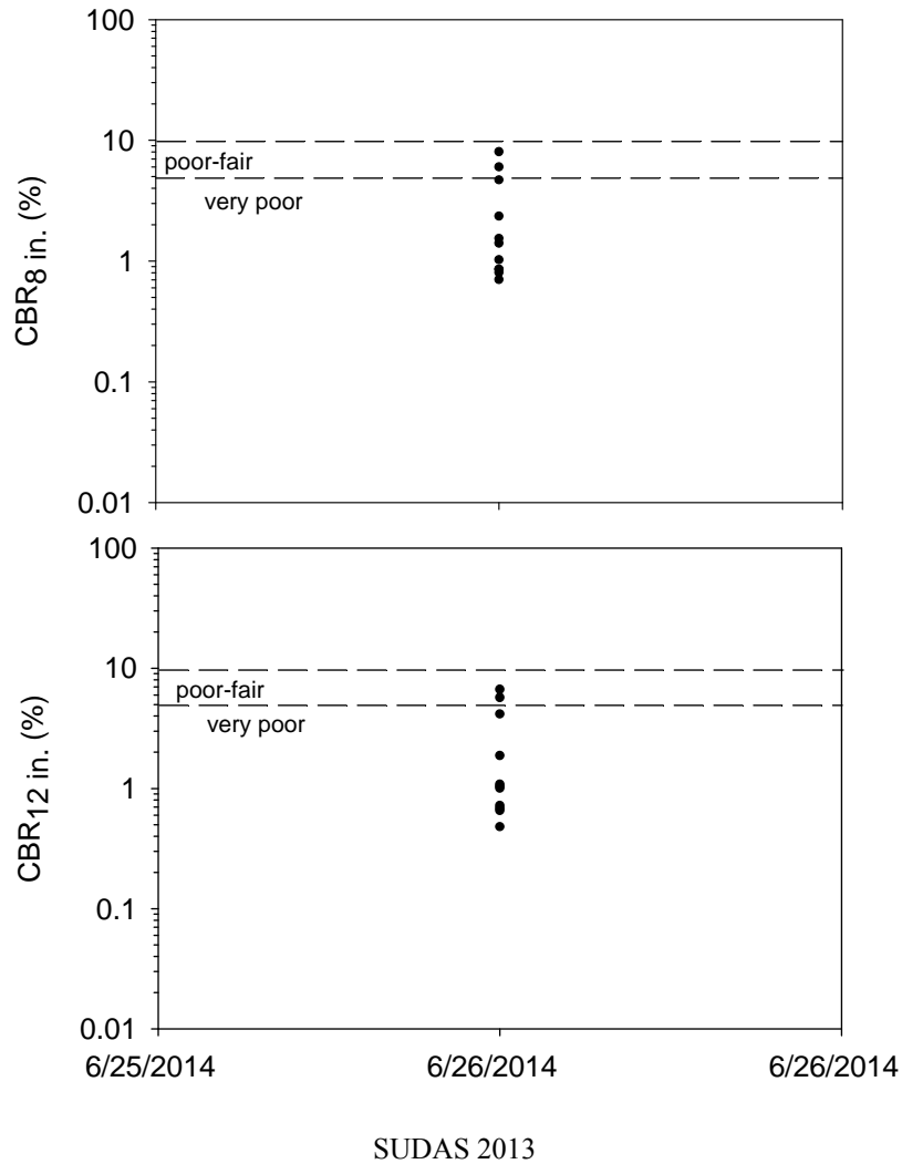
Figure 99. Mills County Project 5: CBR chart with CBR quality rating
