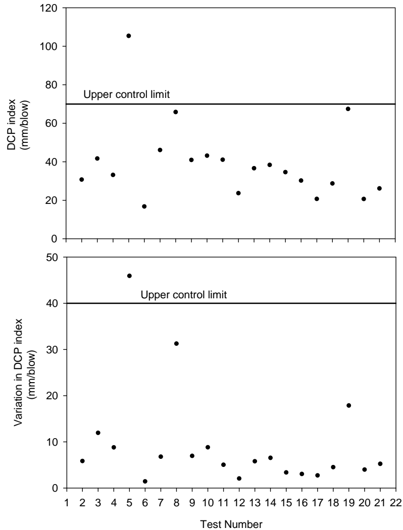
Figure 154. Woodbury County Project 9: Control charts with control limits for DCP index and variation in DCP index
