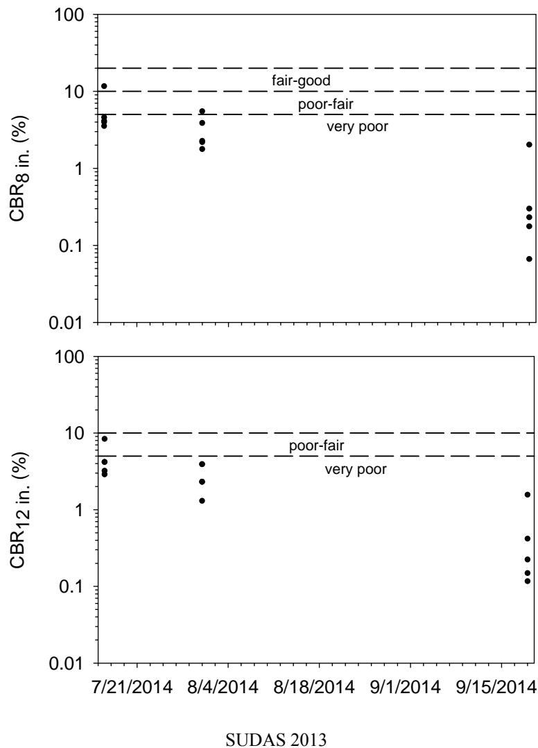
Figure 140. Scott County Project 8: CBR control charts with CBR quality ratings
