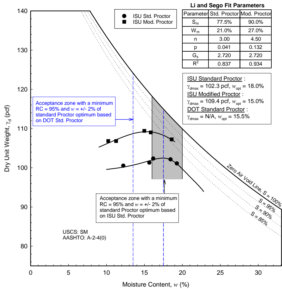
Figure 116. Woodbury County Project 7 TB1: Laboratory Proctor compaction test results with acceptance zone
