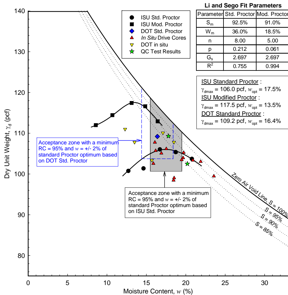
Figure 104. Pottawattamie County Project 6 TB1: Comparison of in situ moisture-density measurements with laboratory Proctor compaction test results and Iowa DOT acceptance limits
