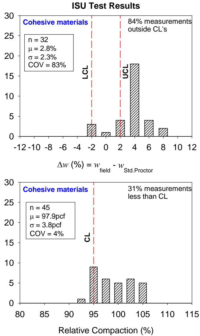
Figure 3. IHRB TR-401 Phase II: Histograms of moisture and relative compaction test results from ISU testing
