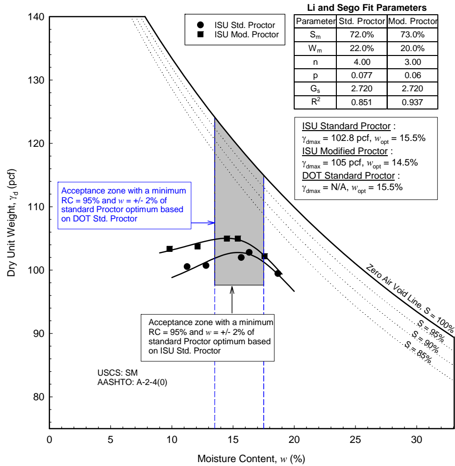
Figure 117. Woodbury County Project 7 TB2: Laboratory Proctor compaction test results with acceptance zone
