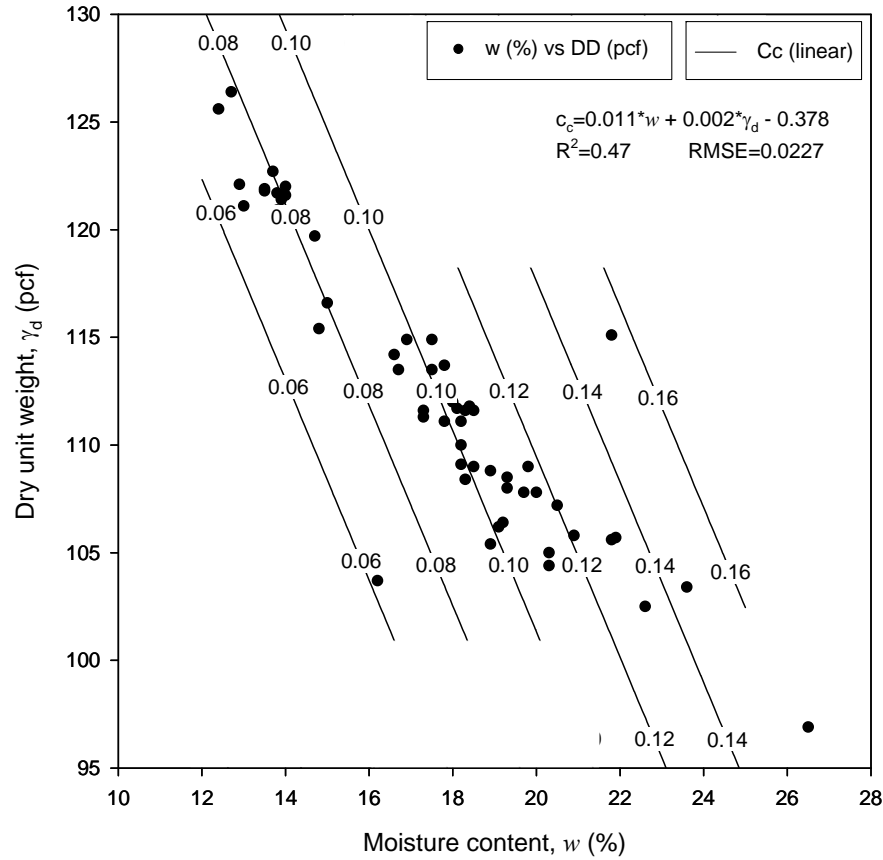
Figure 184. Statistical relationship between moisture content, dry unit weight and compression index for clay
