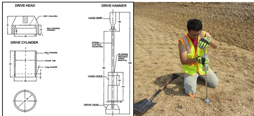
Figure 8. Schematic of drive cylinder (left) and ISU researcher performing in situ testing (right)
