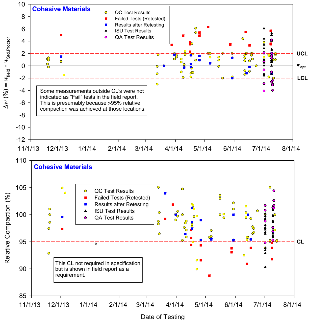
Figure 108. Pottawattamie County Project 6: Moisture control chart
