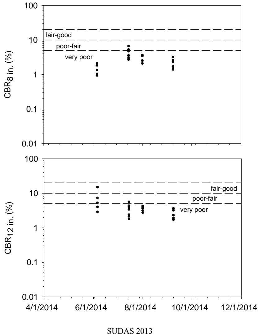
Figure 73. Linn County Project 3: CBR chart with CBR quality rating
