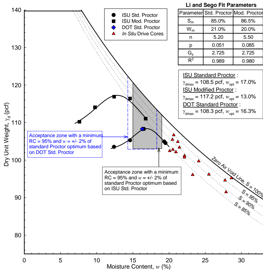
Figure 92. Mills County Project 5 TB1: Comparison of in situ moisture-density measurements with laboratory Proctor compaction test results and Iowa DOT acceptance limits
