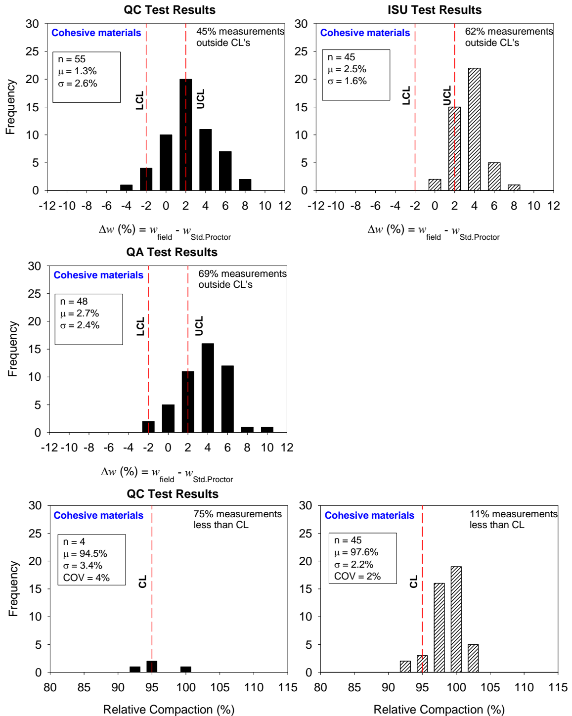
Figure 138. Scott County Project 8: Histograms of moisture control results
