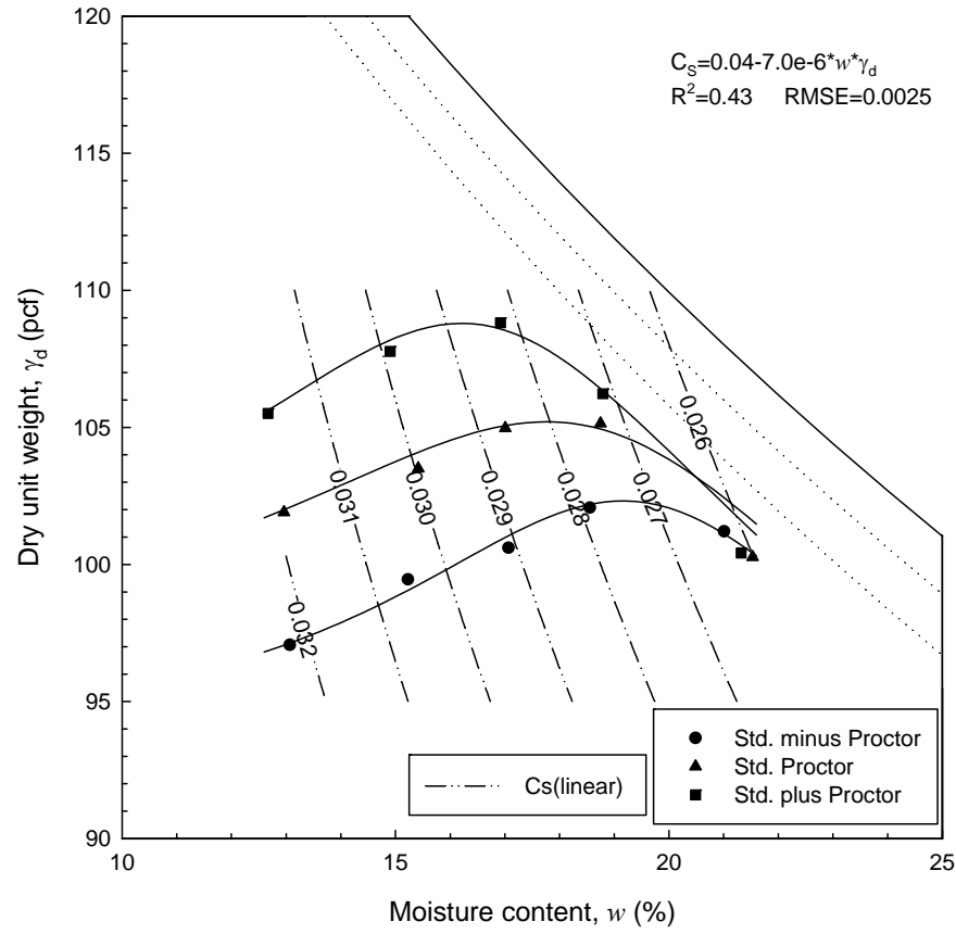
Figure 183. Statistical relationship between moisture content, dry unit weight and swelling index for Iowa loess
