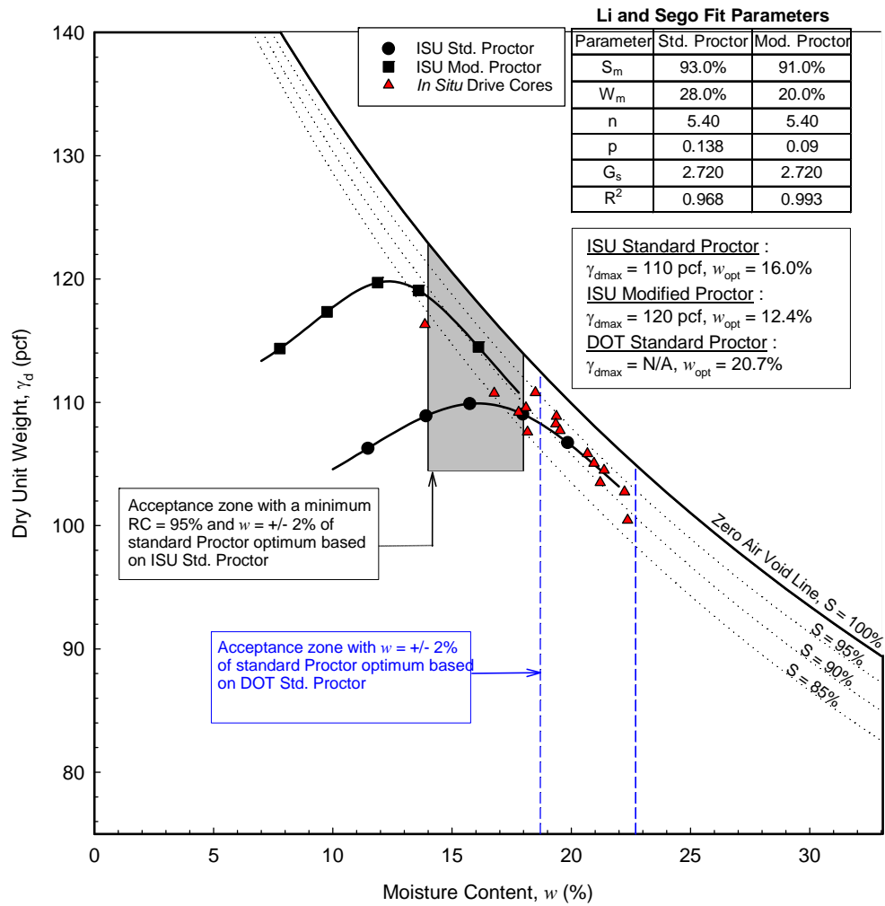
Figure 148. Woodbury County Project 9 TB3: Comparison of in situ moisture-density measurements with laboratory Proctor compaction test results and Iowa DOT acceptance limits
