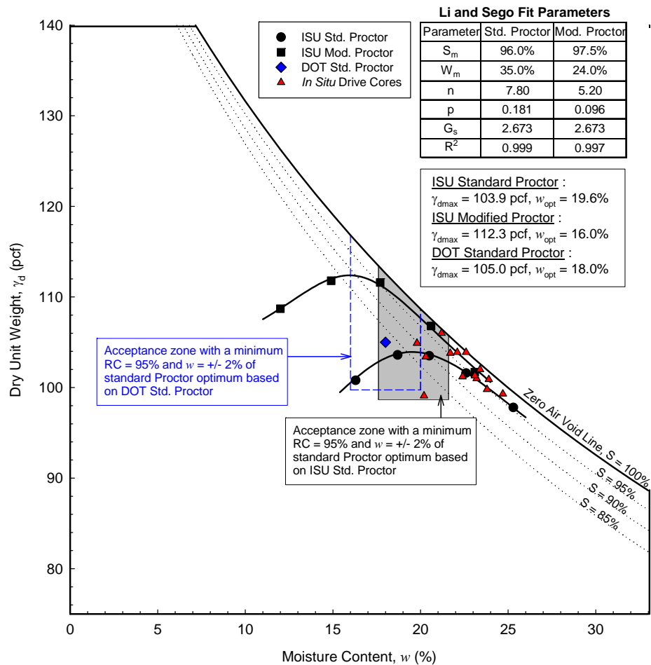
Figure 28. Polk County Project 1 TB1: Comparison of in situ moisture-density measurements with laboratory Proctor compaction test results and Iowa DOT acceptance limits
