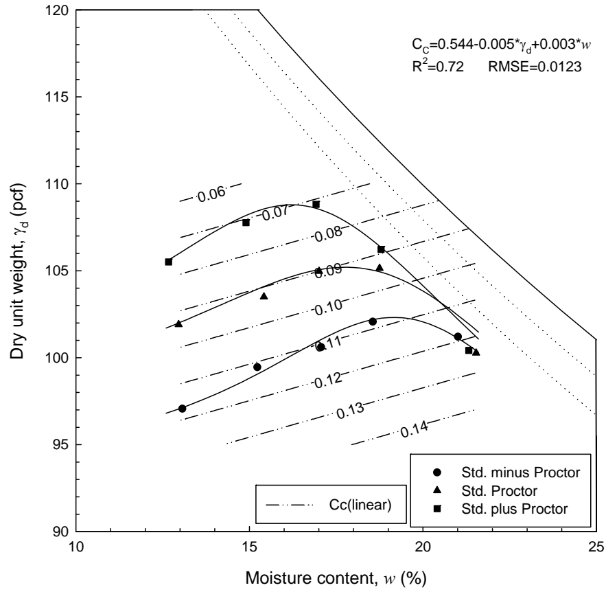
Figure 182. Statistical relationship between moisture content, dry unit weight and compression index for Iowa loess
