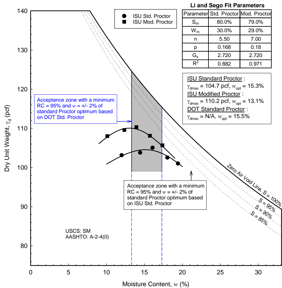
Figure 118. Woodbury County Project 7 TB3: Laboratory Proctor compaction test results with acceptance zone
