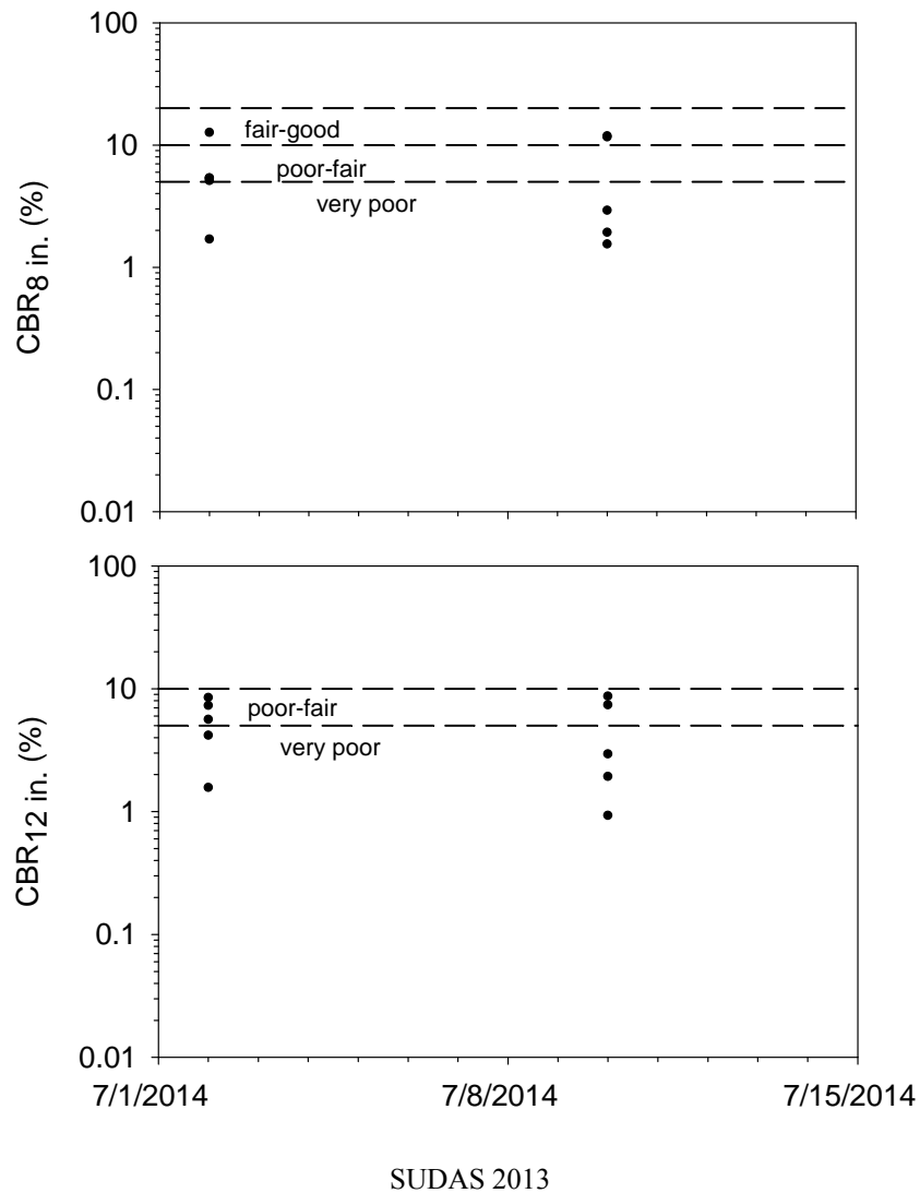
Figure 111. Pottawattamie County Project 6: CBR control charts with CBR quality ratings
