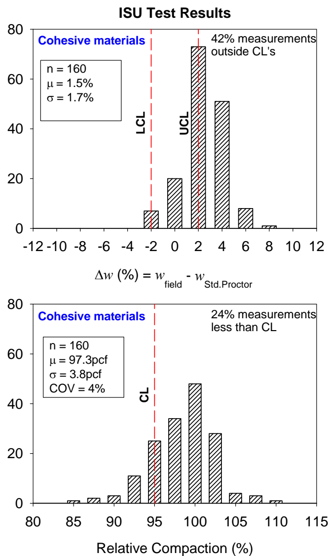
Figure 4. IHRB TR-401 Phase III: Histograms of moisture and density test results
