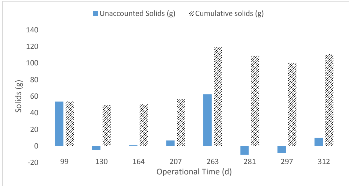
Figure 4.9: Overall solids accumulation in the laboratory-scale SGBR system
