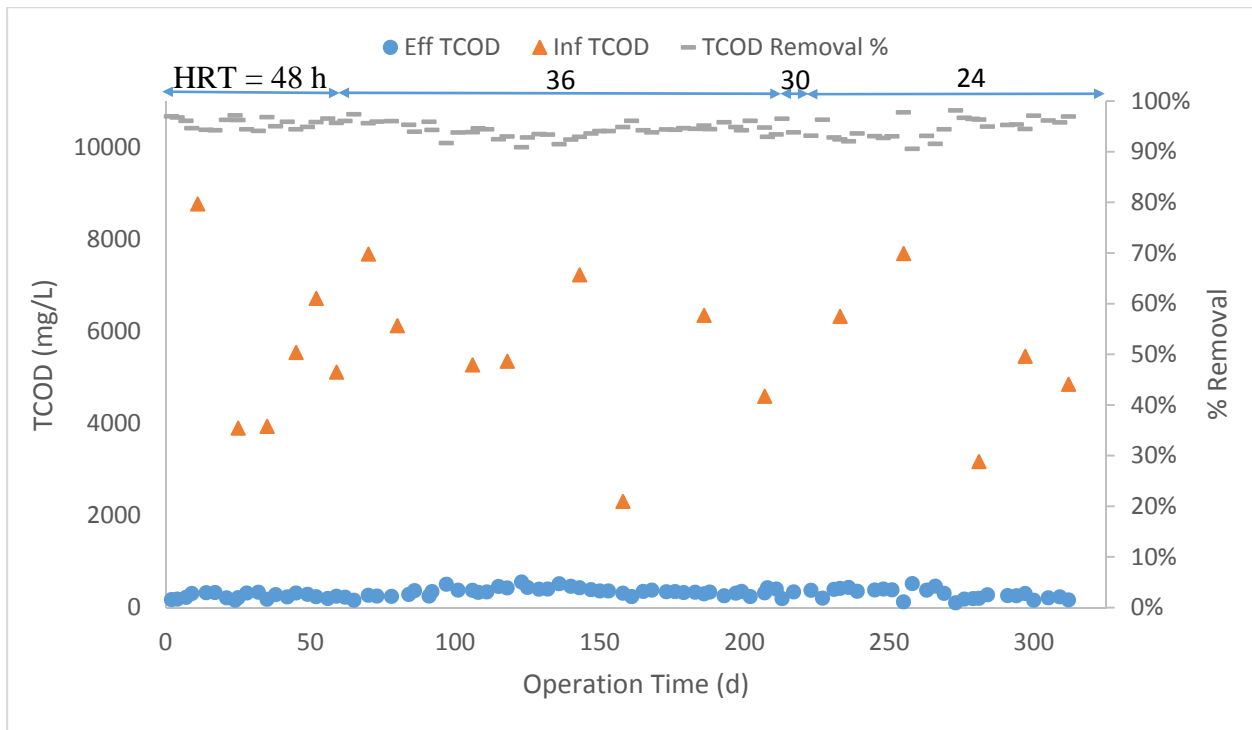
Figure 4.1: Laboratory-scale SGBR TCOD removal
