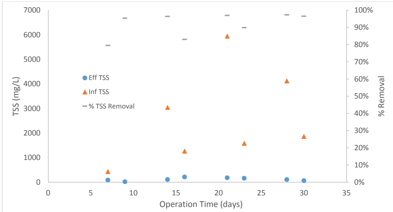
Figure 5.2: Pilot-scale SGBR TSS removal
