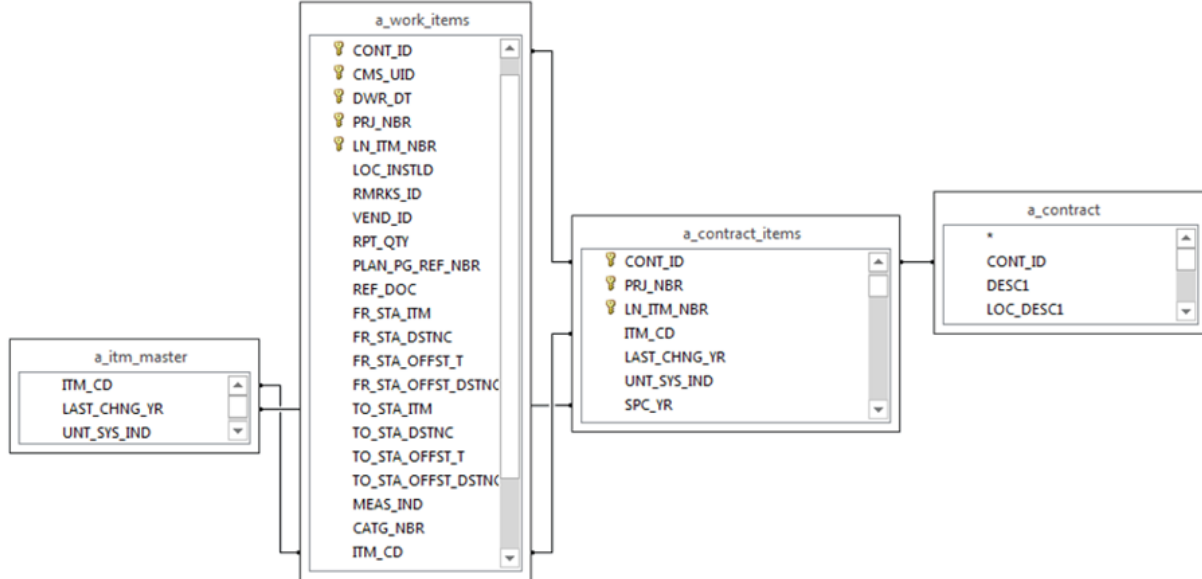
Figure 31 DWR database for discovering precedence relationships of activities
