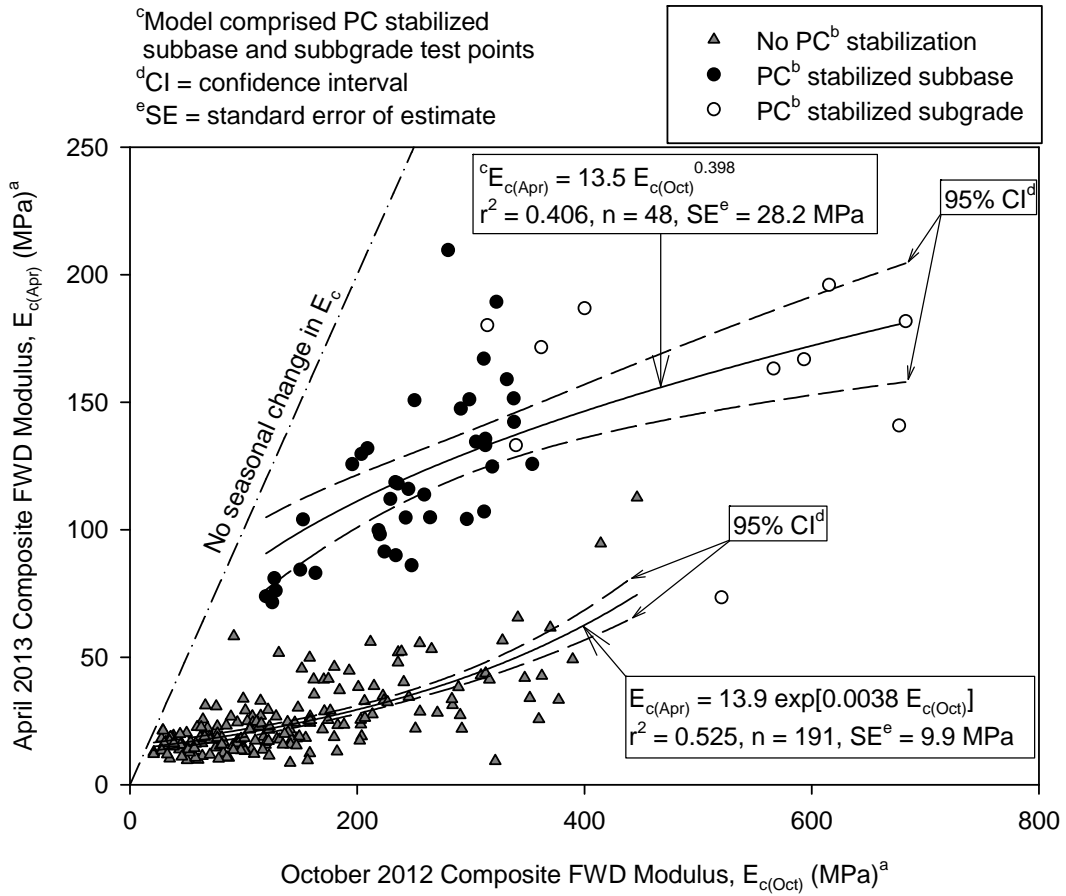
Figure 4.3. Correlations between April 2013 composite FWD moduli and October 2012 composite FWD moduli
