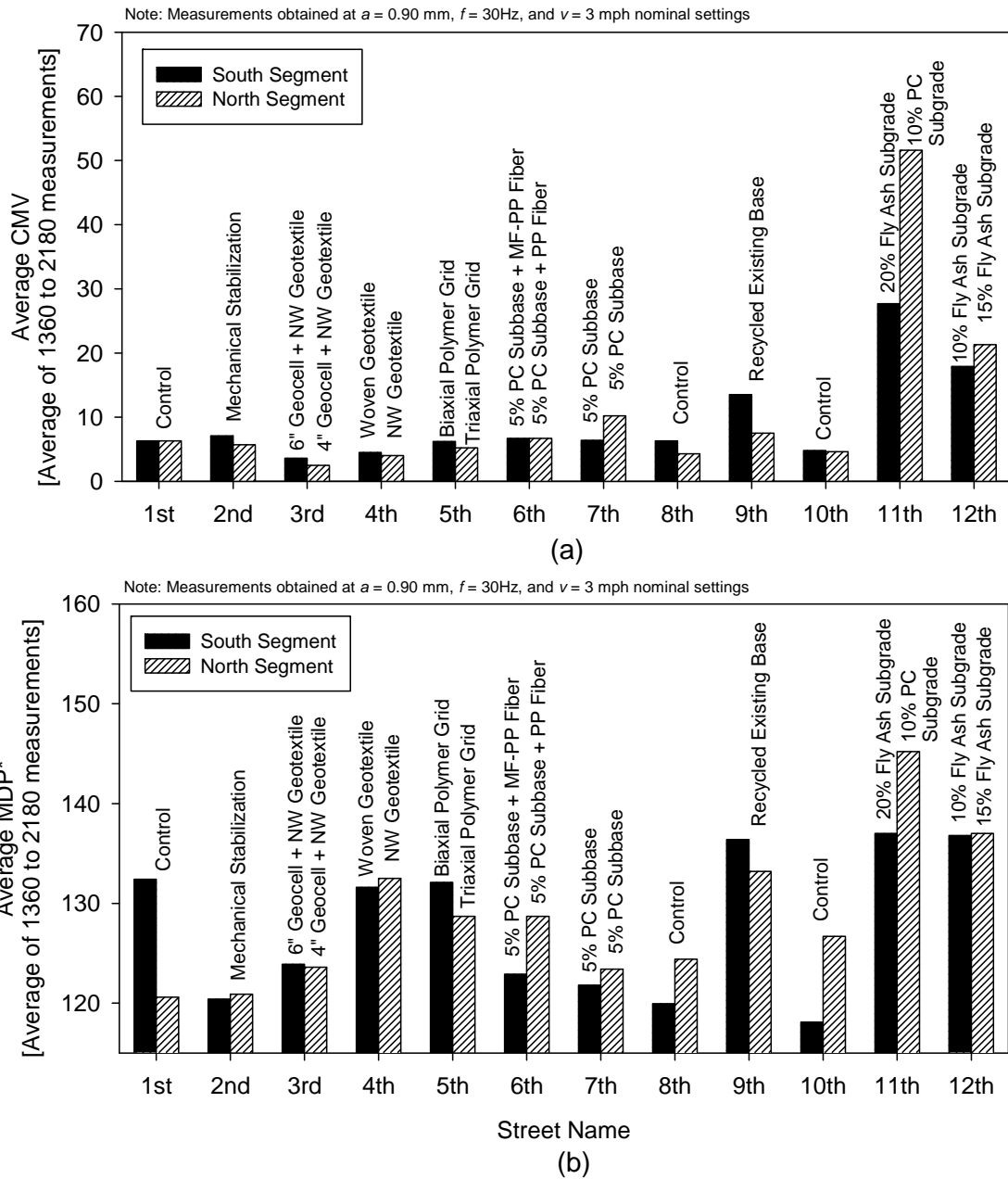
Figure 3.6. RICM results of each test segment: (a) average CMV and (b) average MDP*.
