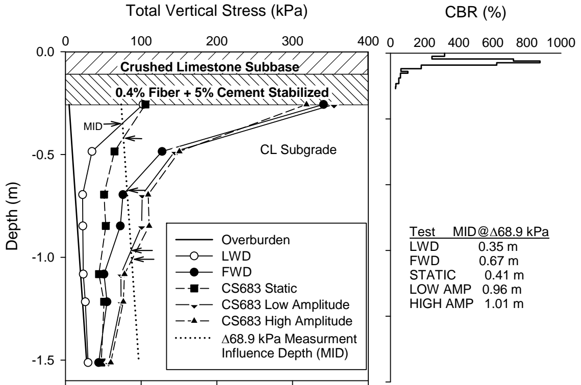
Figure 3.2. Measurement influence depth (MID) for LWD, FWD, and smooth drum roller using +10 psi criteria from piezoelectric earth pressure cells.
