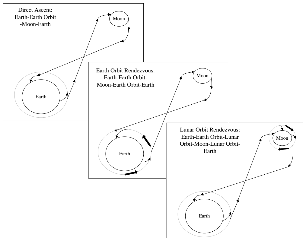
Figure 6.2. Possible Mission-Mode Trajectories [5]
