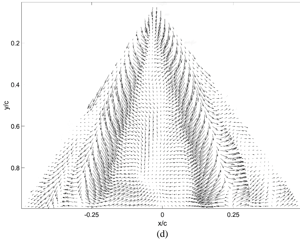
Figure 36: (a) initial image, (b) final image, (c) skin-friction lines, and (d) skin-friction vectors for 55° delta wing at 0° AoA
