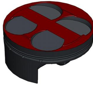
High Compression Flat Surface Piston Design (1mm head clearance with 1mm raised plateau)
