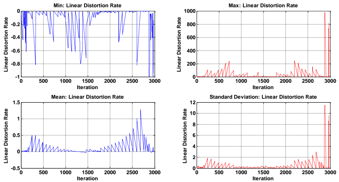
Figure 74. Linear distortion rate for refined simulation
