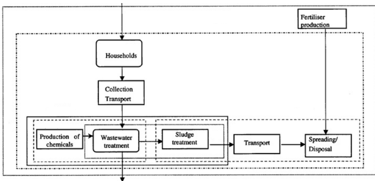
Figure 4. Variation in system boundaries for different LCA studies. Reprinted (adapted) with permission from Lundin et al. (2000). Copyright 2000 American Chemical Society.
