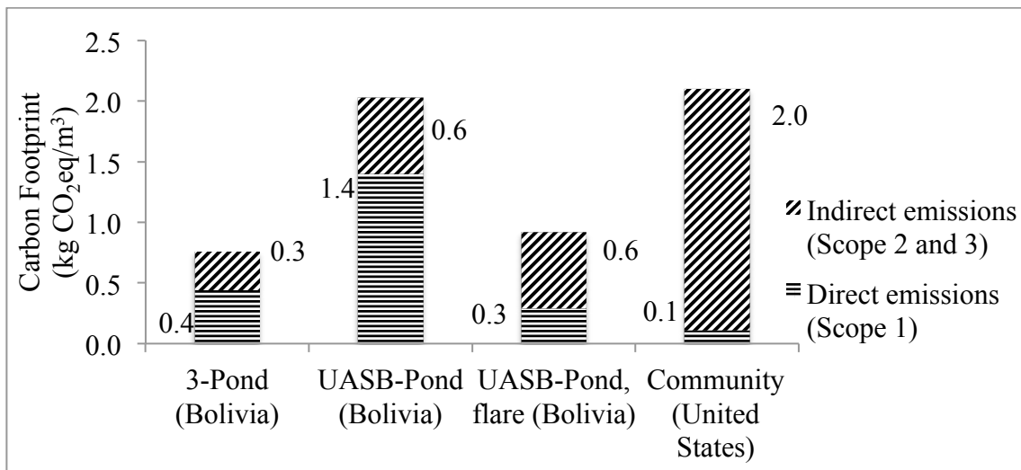
Figure 22. Direct Emissions (Scope 1) and indirect emissions (Scope 2 and 3) contributing to the total carbon footprint of community scale systems in Bolivia and United States
