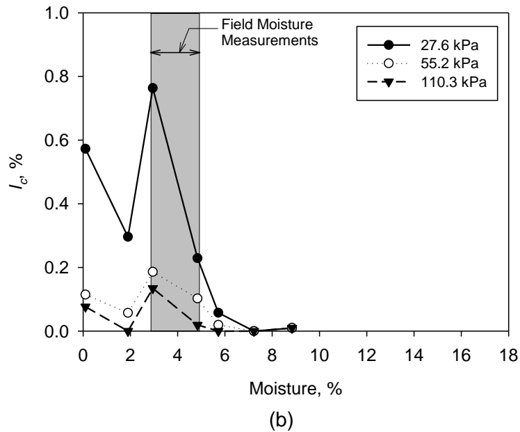
Figure 83. Field moisture results compared to: (a) laboratory compaction results; and (b) laboratory collapse index test results
