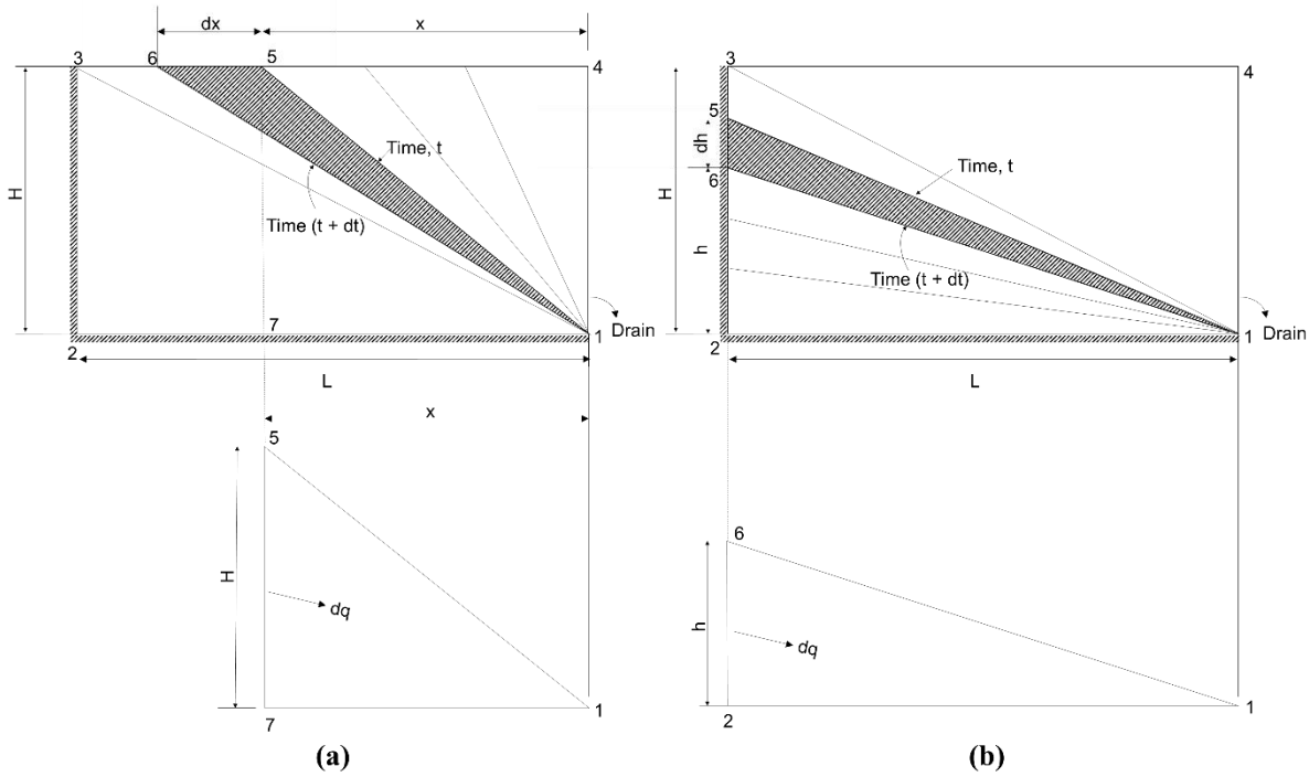
Figure 13. Assumed progress of free water surface: (a) drainage equal to or greater than 50% and (b) drainage equal to or less than 50%(reproduced from Casagrande and Shannon 1952)
