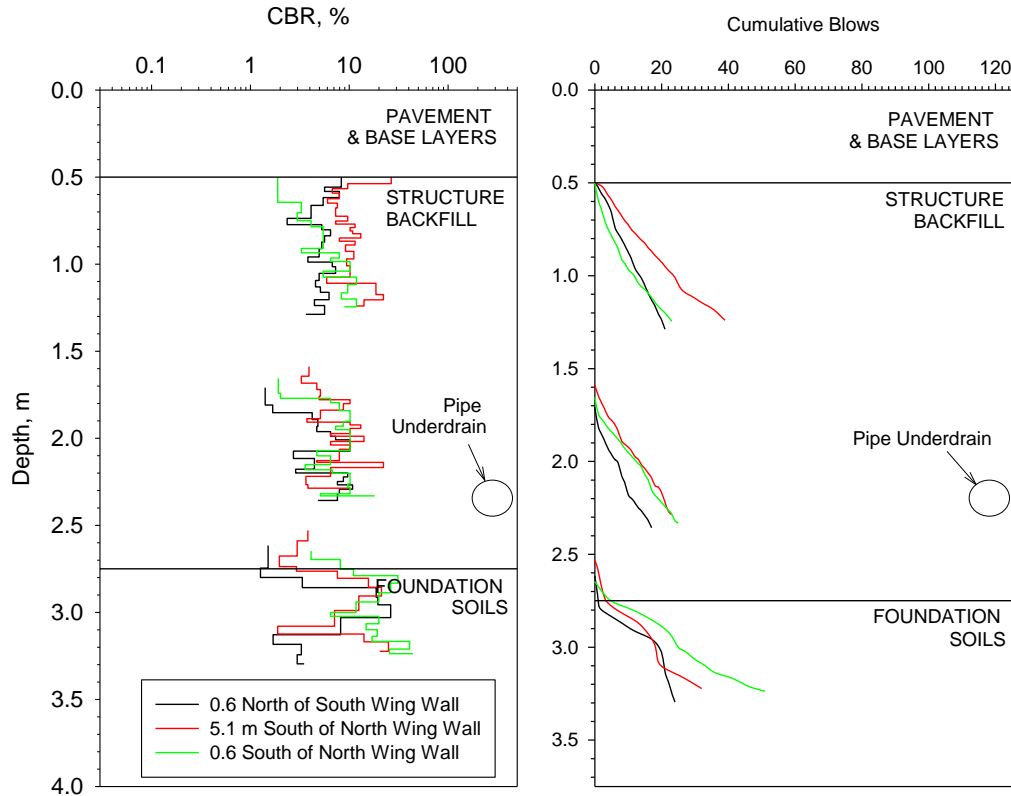
Figure 123. DCP test results for Hobbles Creek Bridge
