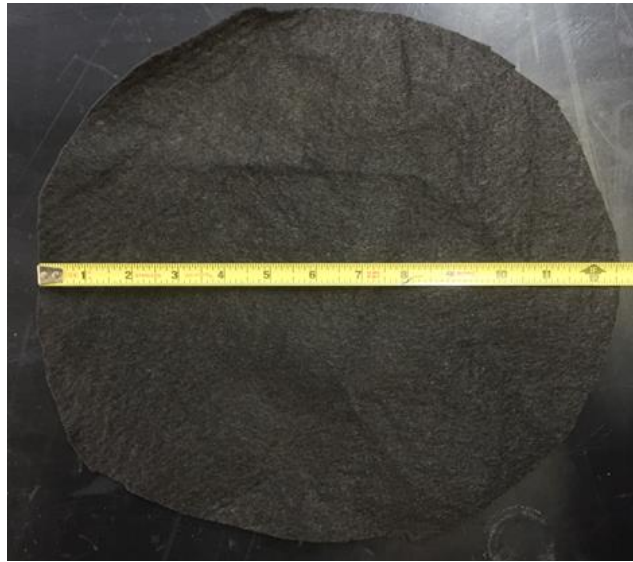
Figure 24. Geosynthetic fabric used in permeability testing
