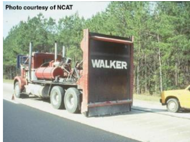
Figure 3 Crack-and-seat
