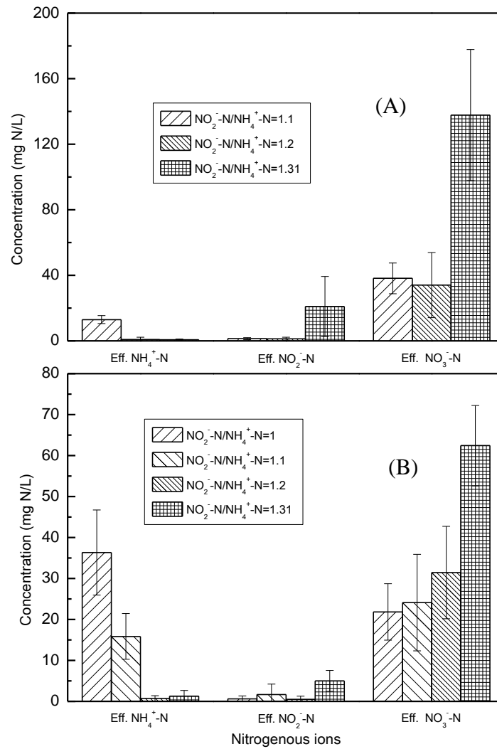
Figure 3.1. Effluent profiles under different influent \text{NO}_2^-/\text{NH}_4^+-\text{N} ratios.
