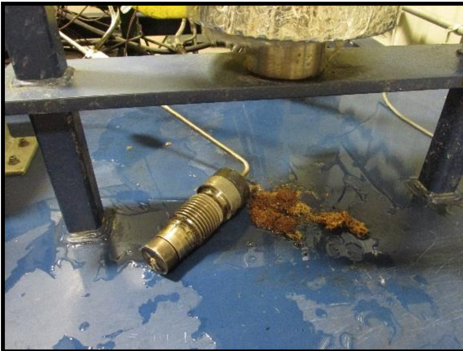
Figure 4.5. Solids that settled out of the SCFR HTL run
