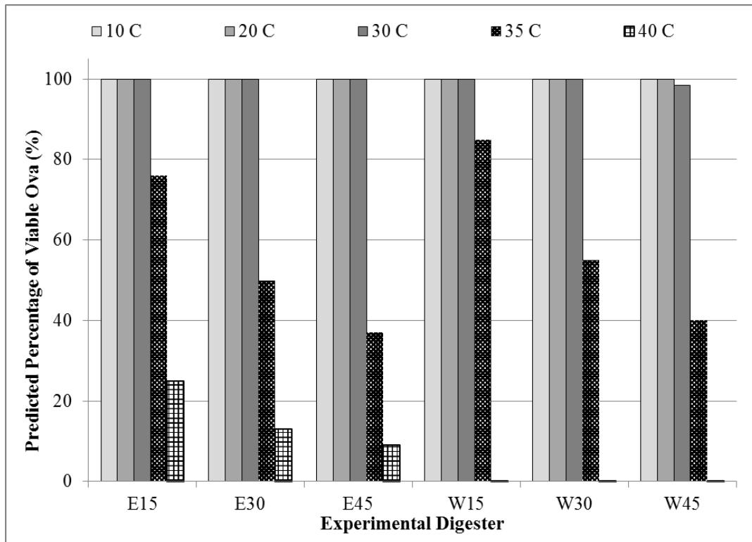
Figure 5.7 – Using t_{99} values from Table 5.1, the estimation of viable ova percentages in the effluent are determined for different digestion temperatures. Based upon the semi-continuous residence time distributions for the experimental digesters, only systems operated above 40 °C and fed weekly are capable of removing 100% of viable ova.
