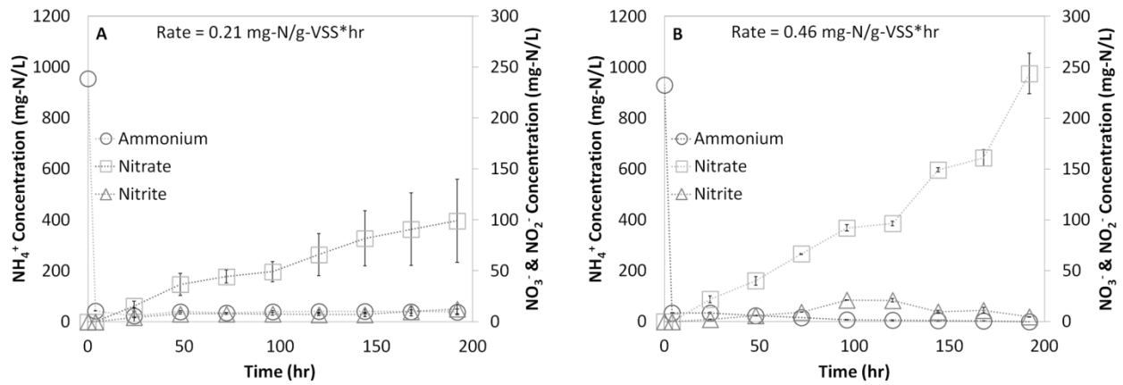
Figure 4-5. Ammonium, nitrite and nitrate concentration during nitrification of 1,000 \text{ mg NH}_4^+\text{-N L}^{-1} with addition of 150 \text{ g L}^{-1} of chabazite; (A) synthetic waste S-1, and (B) real ADSW centrate.
