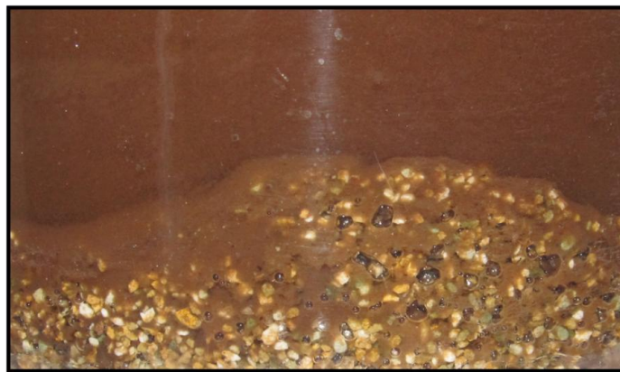
Figure 5-6. Photograph of the chabazite-SBR during the aerobic stage showing zeolite material settling despite mixing.
