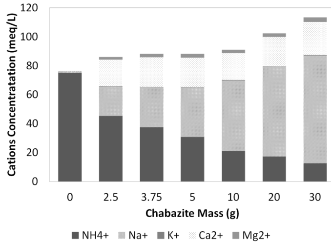
Figure 3-1. Cation concentrations at equilibrium during NH 4 + uptake.
