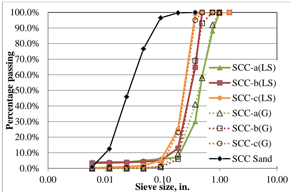
Figure 2. Aggregate gradations.
