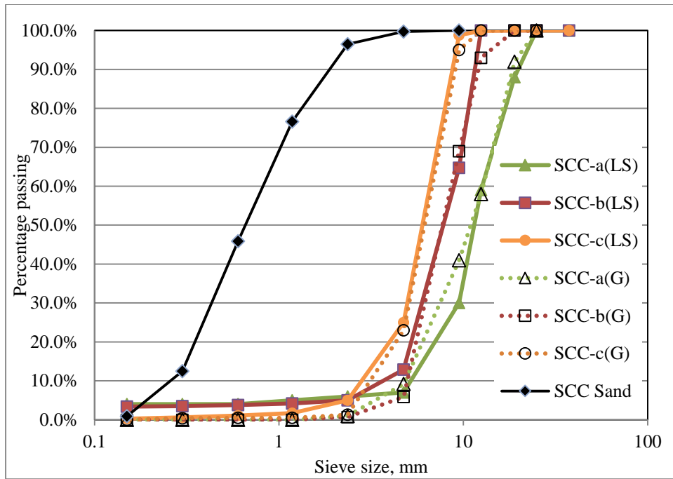
Figure 3. Aggregate gradations.
