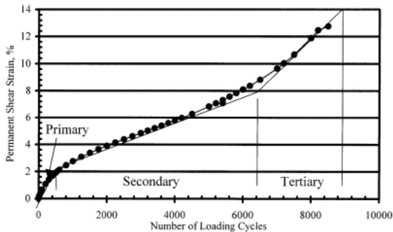
Figure 3.4 Permanent shear strain versus number of loading cycles (Witczak, Kaloush, Pellinen, El-Aasyouny, & Von Quintus, 2002)
