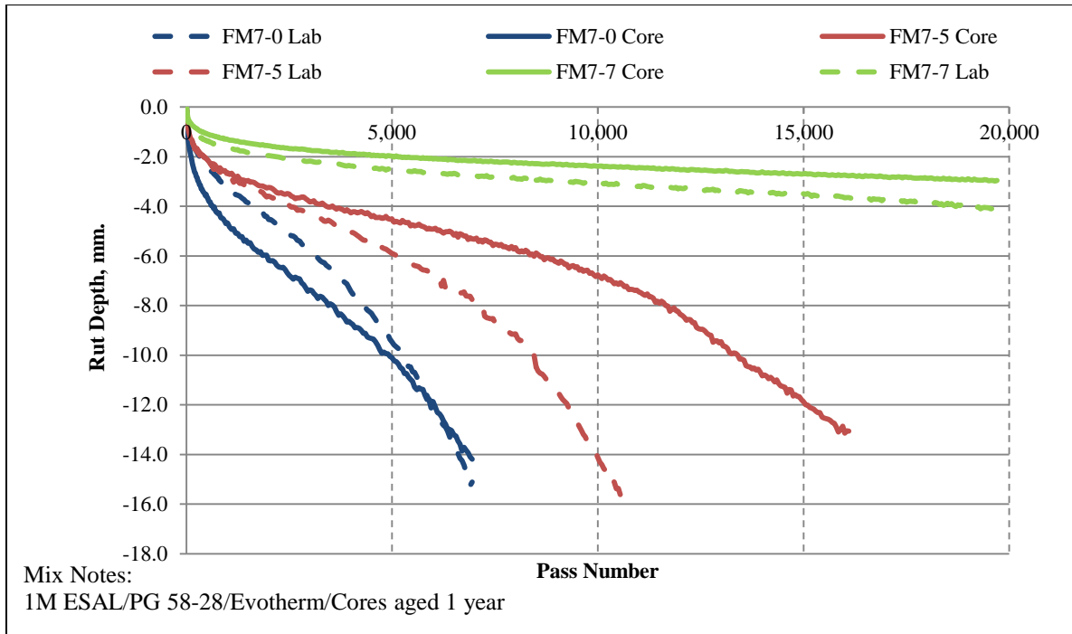
Figure 4.44 FM7 Hamburg rutting depth versus passes (Evotherm with 0%, 5%, and 7% Shingles)
