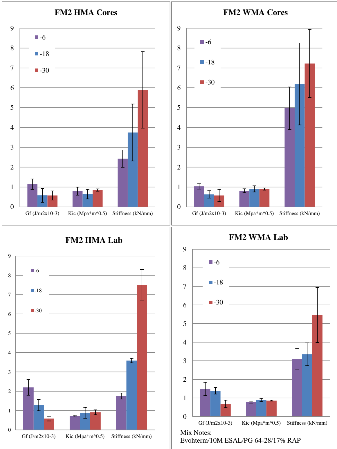
Figure 4.22 SCB results for FM2 (HMA/Evothertm) (Average core air voids are HMA=7.6% and WMA=8.6%; pavement cored after 2 years of service life)
