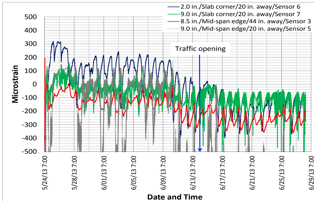
Figure 3-29. Strain measurement.
