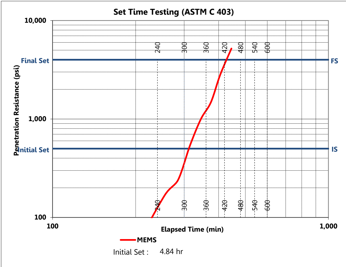
Figure C-1. Set time test (ASTM C403)
