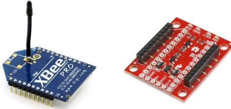
Figure 6: XBee-PRO (left) and XBee Explorer Regulated (right)
