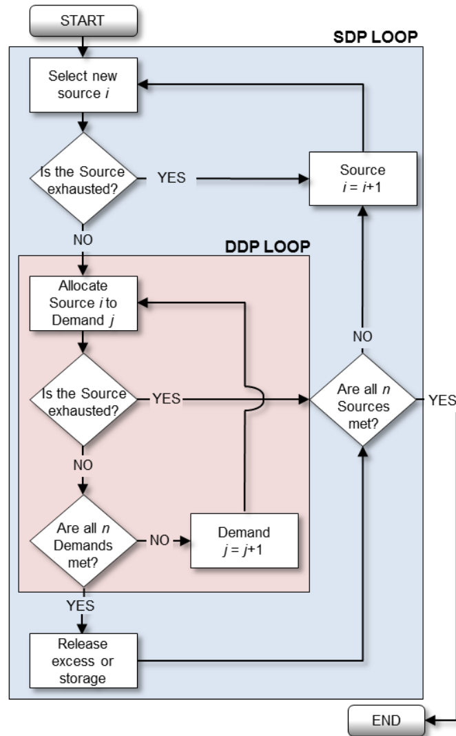
Figure 4.1: Nested prioritization algorithm – demand-driven prioritization (DDP) is nested within source-driven prioritization (SDP).
