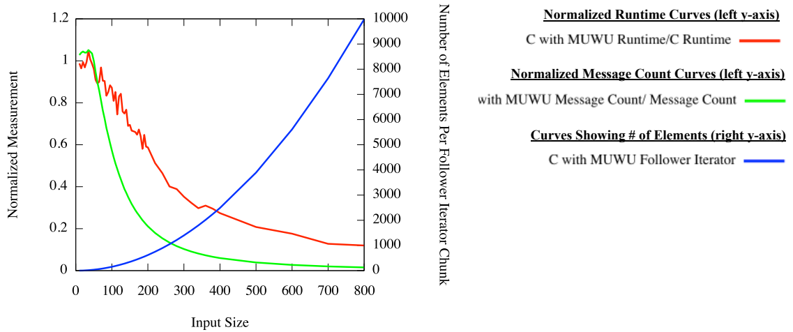
Figure 8.11: ftdt-2d weak scaling results.
