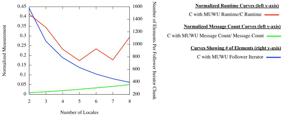
Figure 8.5: folding strong scaling results.
