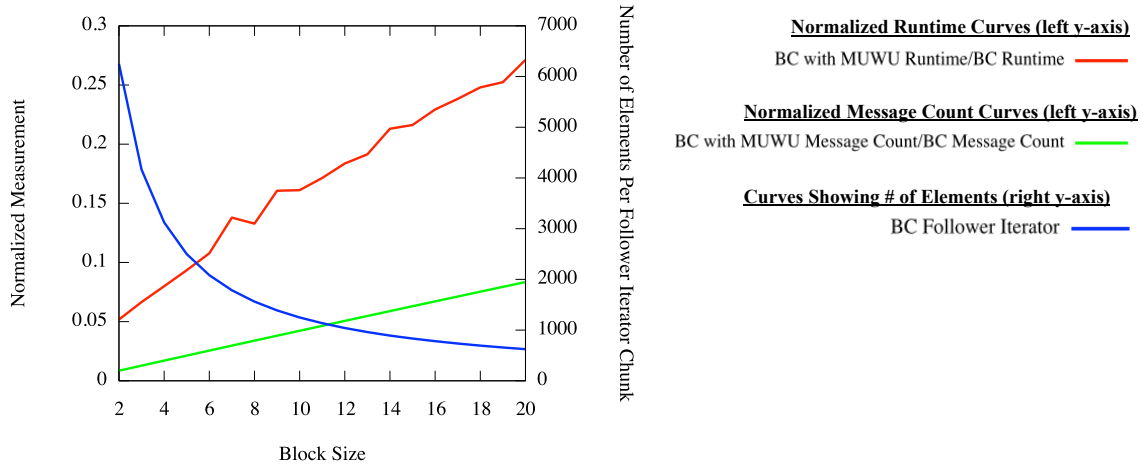
Figure 8.12: folding block size variation results.
