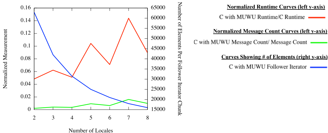
Figure 8.7: ftdt-2d strong scaling results.
