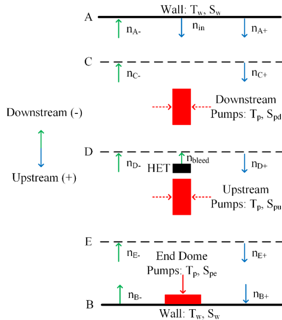
Figure 5.2: Updated background flow model representation of VTF-2 to account for axial bleed flow injection.
