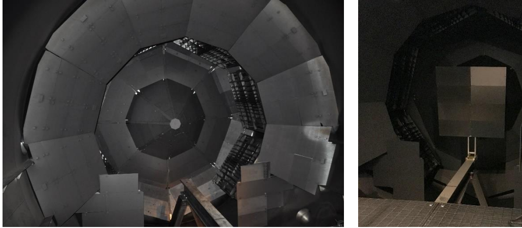
(a) (b) Figure 4.16: (a) Conic and (b) flat plate beam dump configurations for VTF-2.
