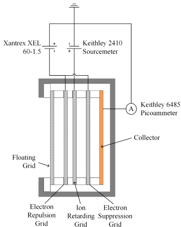
Figure 4.7: Schematic of the RPA measurement circuit.
