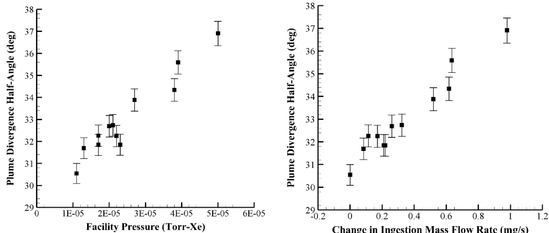
(a) (b) Figure 6.2: H6 plume divergence half-angle as a function of (a) facility pressure (b) ingestion mass flow rate.
