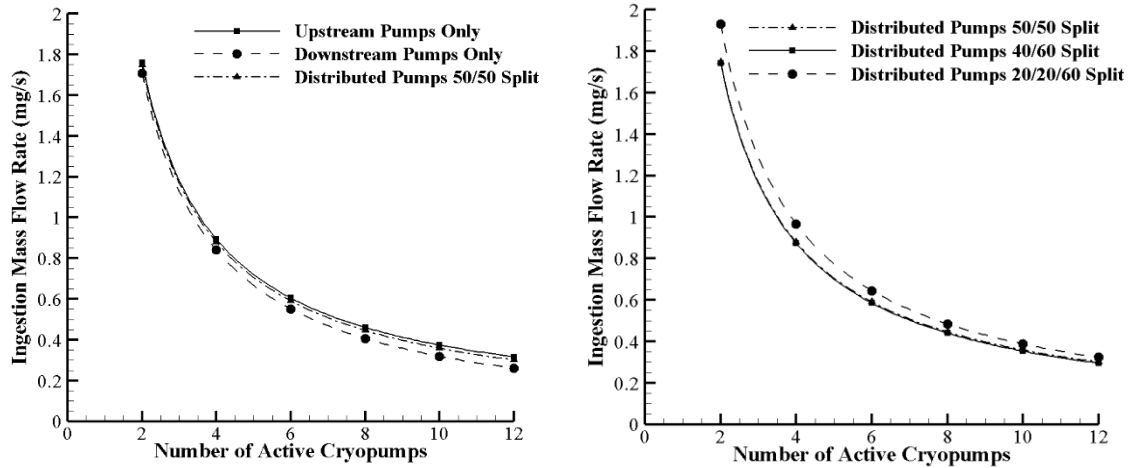
(a) (b) Figure 3.7: Ingestion mass flow rate of the P5 operating at an anode flow rate of 15 mg/s comparing: (a) upstream, downstream, and distributed pumps and (b) different distributed pump configurations.
