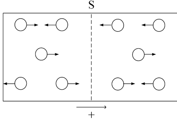
Figure 2.2: One-dimensional motion of a rarefied gas.
