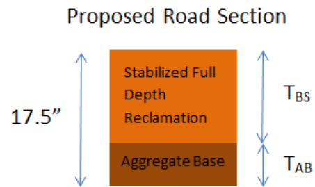
Figure 31: Diagram to show the proposed road section expressed in terms of GE values
