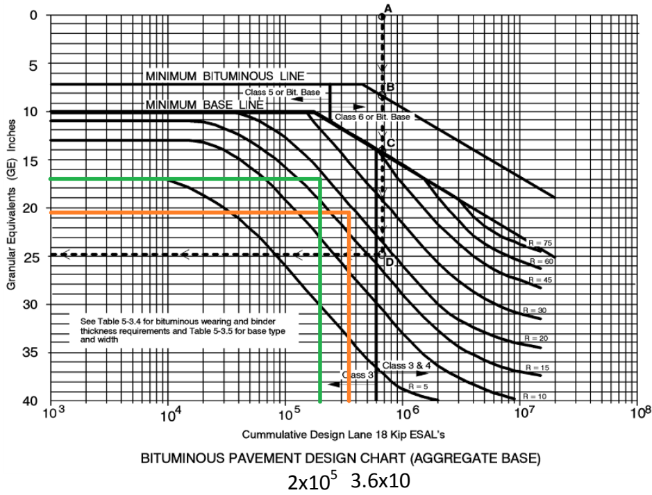
Figure 33: Bituminous Pavement Design Chart to calculate the Total GE values required for 200,000 and 367,000 ESALs and R-value of 18
