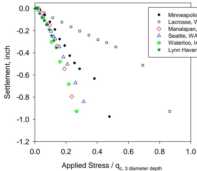
Figure 96. The results of combination in situ CPT results in matrix soil and single IRAP load test results
