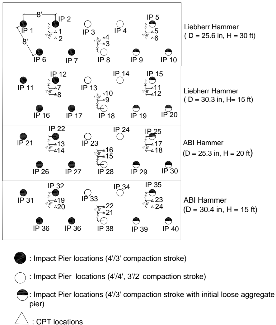
Figure 67. Waterloo, IA (Liquefaction): Pier and CPT locations plan layout
