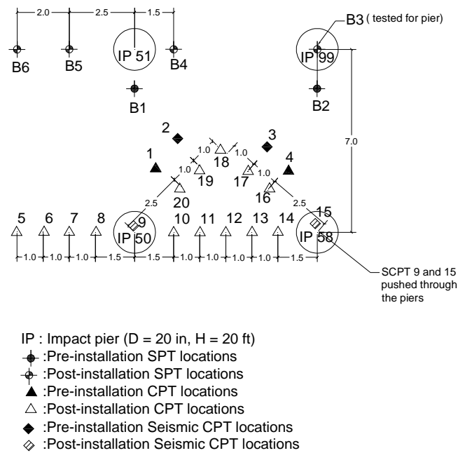
Figure 34. Tampa, FL: Pier and CPT locations plan layout
