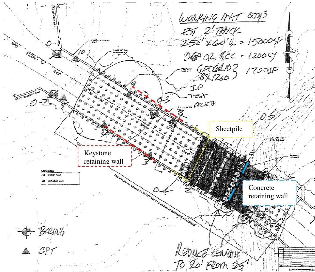
Figure 27. Lacrosse, NJ: Project plan layout (French Parrello Company)
