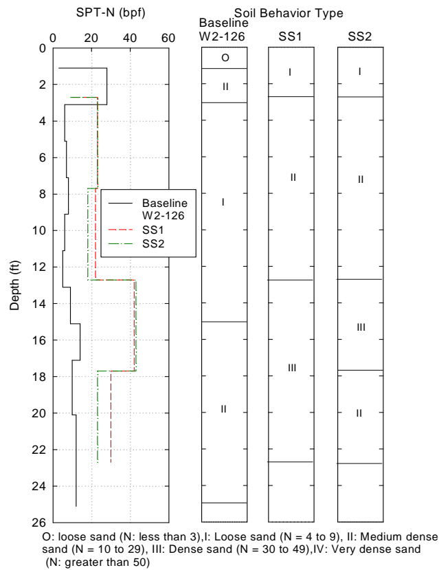
Figure 72. Rochester, NH: Pre-installation and post-installation SPT profiles
