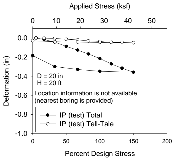
Figure 61. Jacksonville, FL: Modulus load test results on trial pier at vicinity B-2 location
