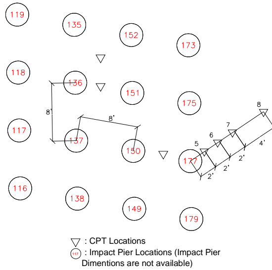
Figure 28. Manalapan, NJ: Plan layout of the CPT locations
