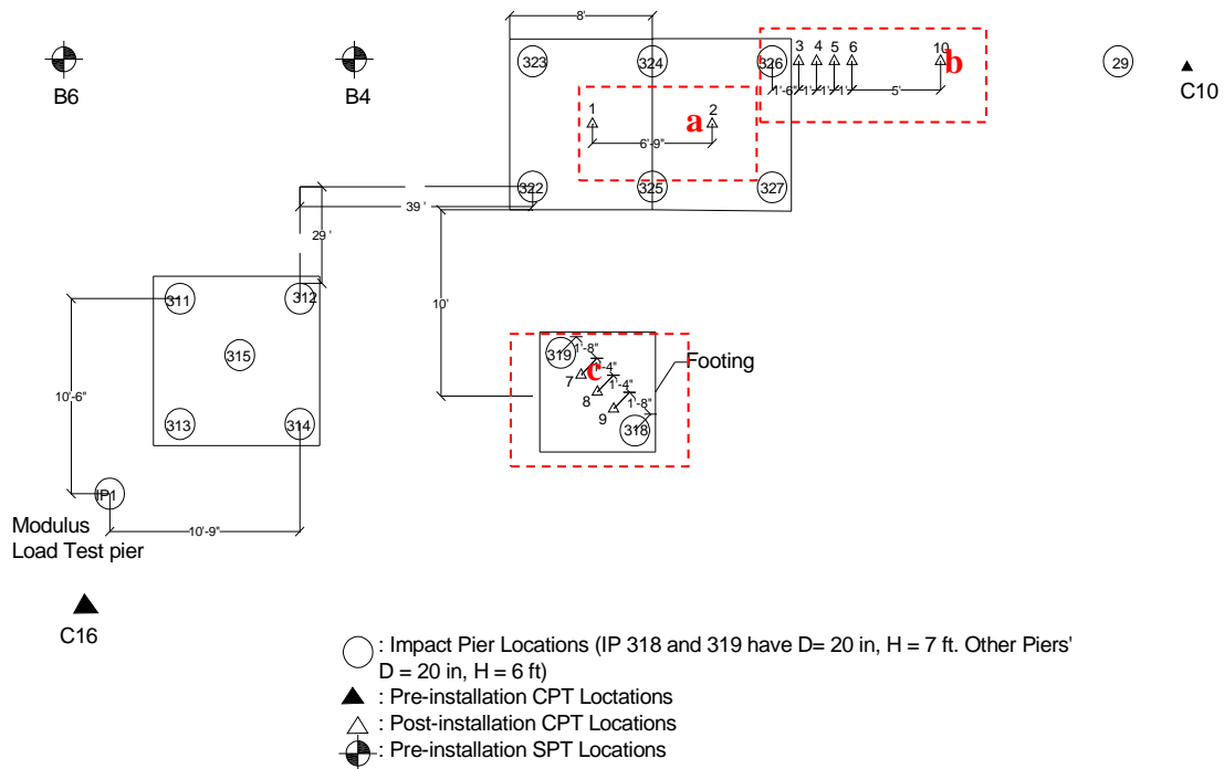
Figure 56. Lynn Haven, FL: Pier and CPT locations plan layout
