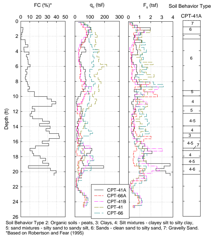
Figure 44. Springfield, MA: CPT profiles performed on center on piers and matrix soil (only CPT 41A performed in the matrix soil)
