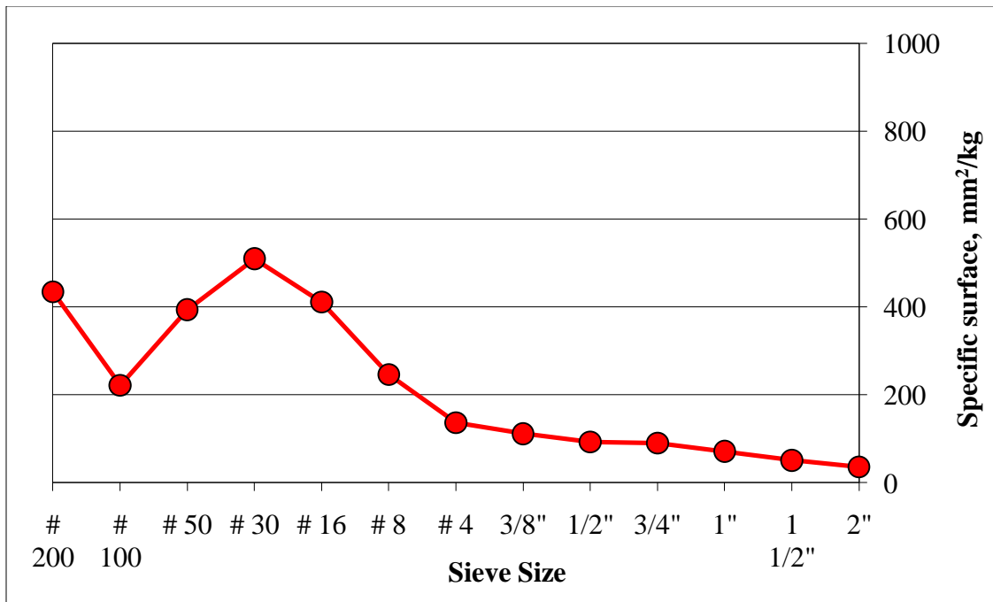
c) Specific surface chart
