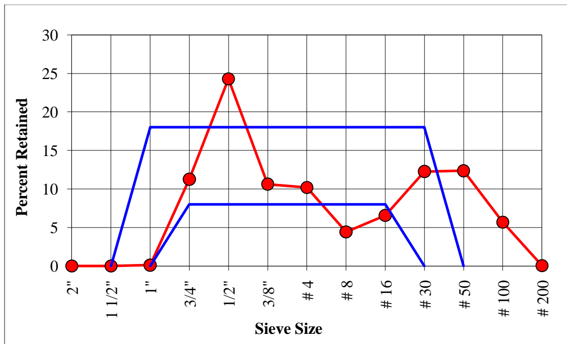
e) 8/18 gradation chart
