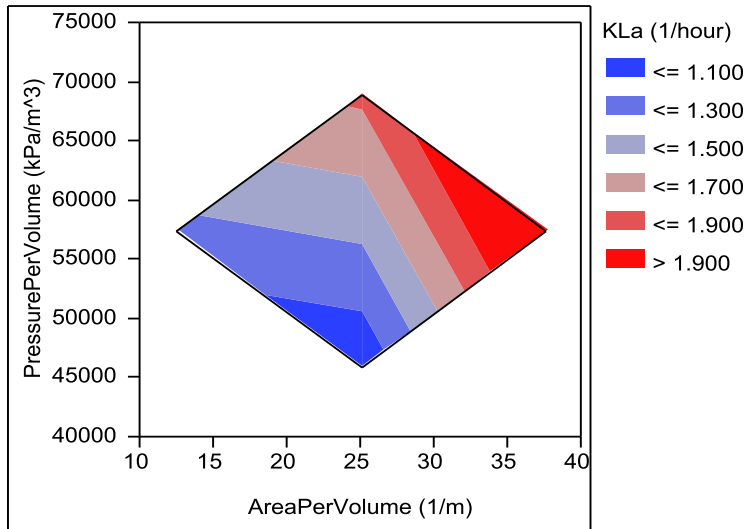
Figure 8. Contour plot for K_{La} for interaction of PressurePerVolume and AreaPerVolume with PowerPerVolume=874 W/m 3
