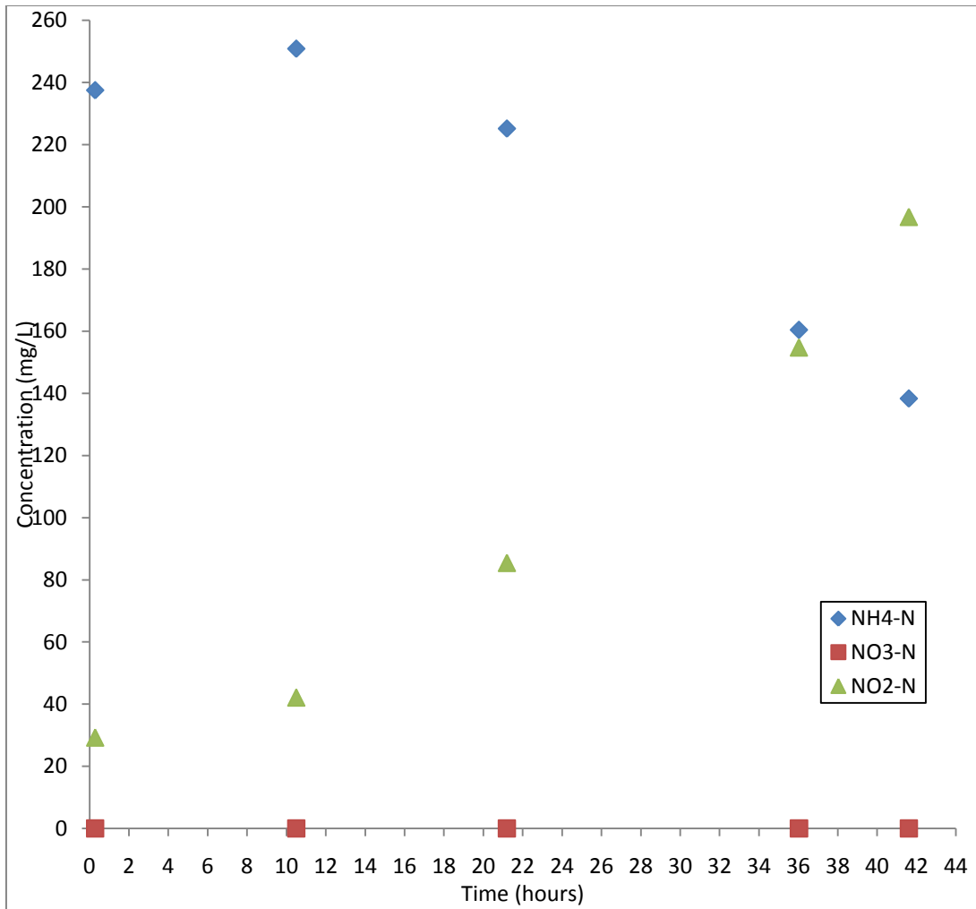
Figure 22. Nitrogen profile of partial nitrification reactor after 26 days of operation. ◆: NH 4 + -N; ■: NO 3 - -N; ▲: NO 2 - -N
