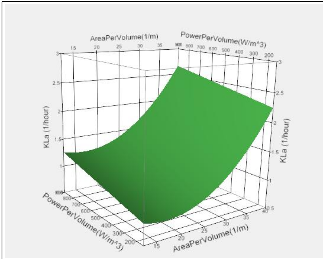
Figure 17. Response surface simplified model PowerPerVolume: 531.5 W/m 3 , AreaPerVolume: 25.15 m 2 /m 3 , PressurePerVolume: 57456 kPa/ m 3
