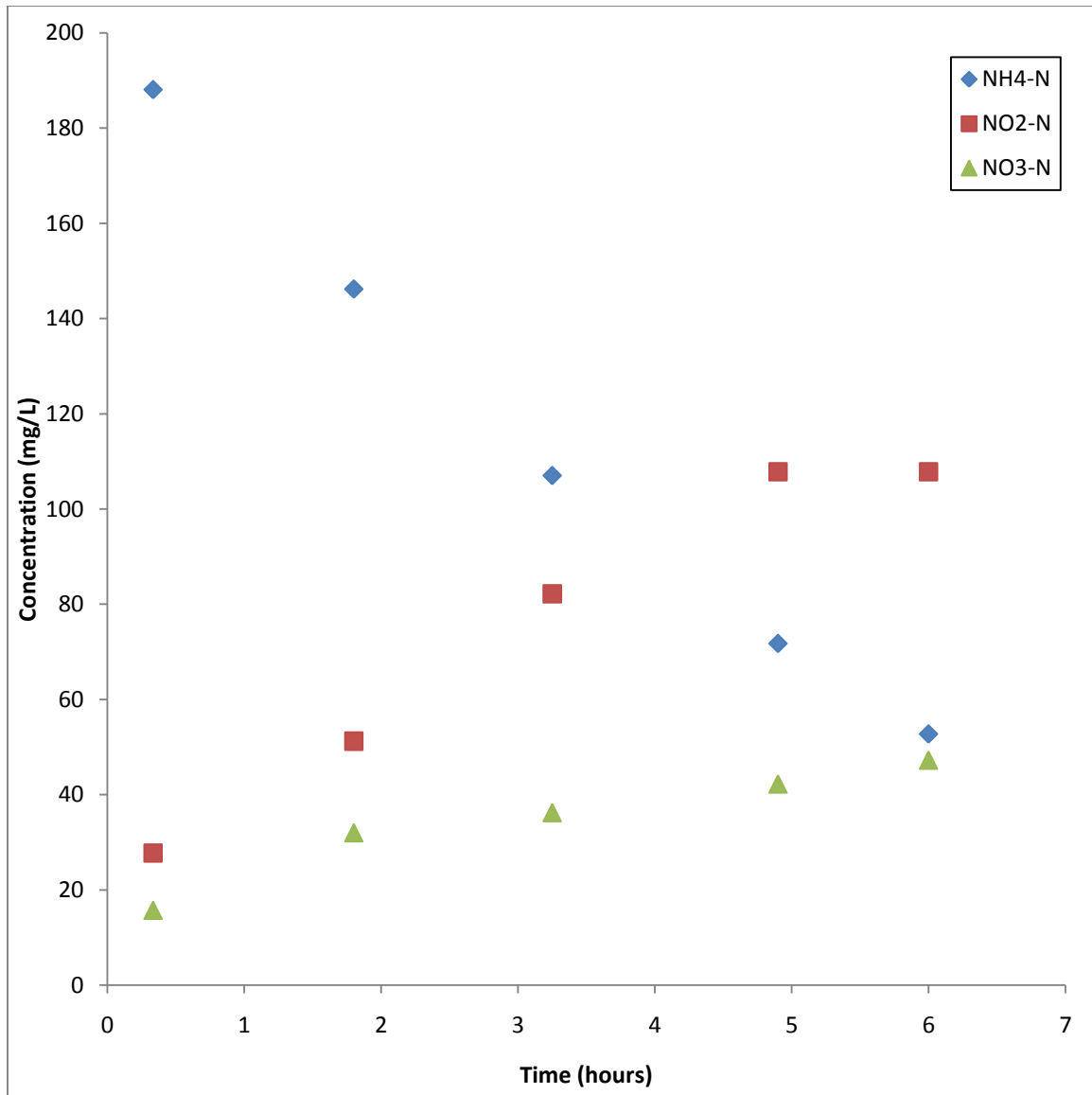
Figure 27. Partial nitrification utilizing a polypropylene membrane aeration system. ◆: \text{NH}_4^+\text{-N} ; ■: \text{NO}_2^-\text{-N} ; ▲: \text{NO}_3^-\text{-N}
