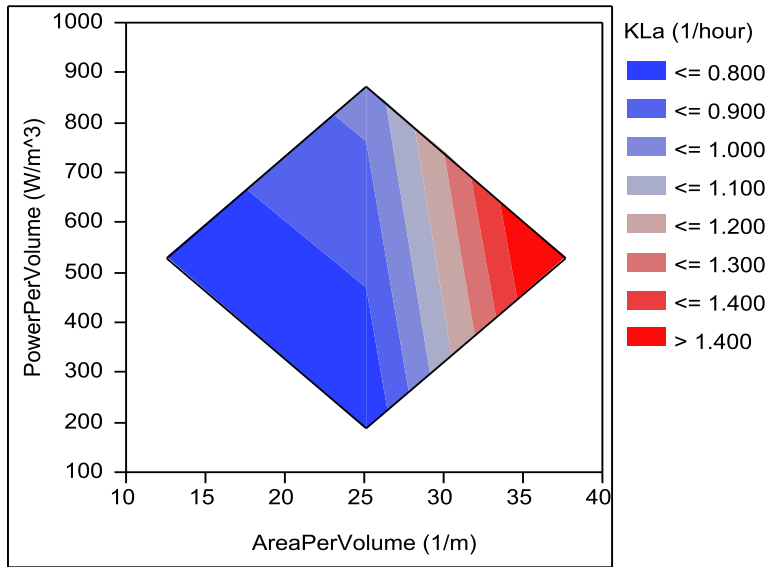
Figure 9. Contour plot for K_{La} for interaction of PowerPerVolume and AreaPerVolume with PressurePerVolume=45965 kPa/ m 3
